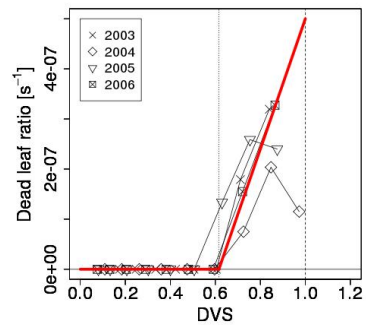
Figure 3. Ratio of dead leaf. A red line is fitted. DVS: development stage
