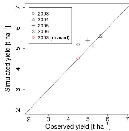
Figure 12. Comparison of yields between simulations and observations
