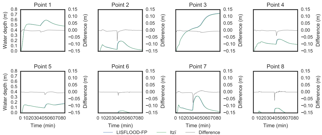
Figure 7. Comparison of water depths at control points
