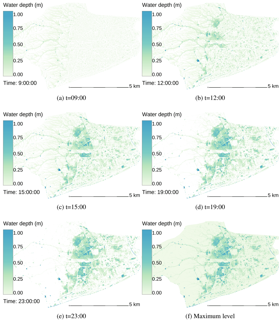
Figure 13. Evolution of water depth in Hull when using a uniform friction
