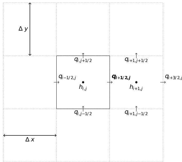
Figure 2. A 2D view of the staggered grid used by the numerical scheme.
