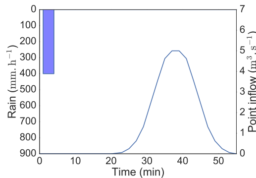
Figure 5. Rectangular hyetograph and inflow hydrograph for the EA test 8a
