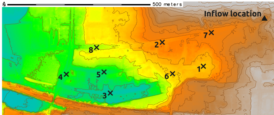
Figure 6. DEM of EA test 8a with control and inflow points
