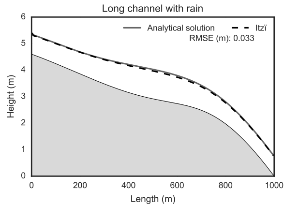
Figure 4. One-dimensional MacDonald long-channel with rain
