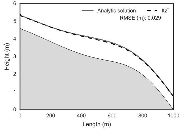
Figure 4. Comparing Itzi with an analytic solution. Case of the one-dimensional MacDonald long-channel with rain.
