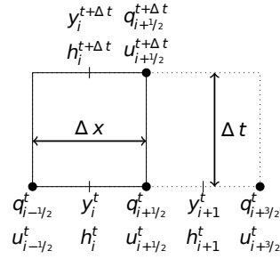
Figure 1. Grid and variables used in the numerical scheme. Time is shown in the vertical axis. Variables at the bottom are used at time t to calculate variables at the top at time t + \Delta t .
