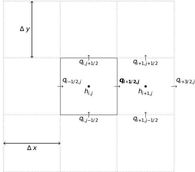
Figure 2. A 2D view of the staggered grid used by the numerical scheme. The variable in bold will be calculated at t + \Delta t using all the displayed variables values at time t .
