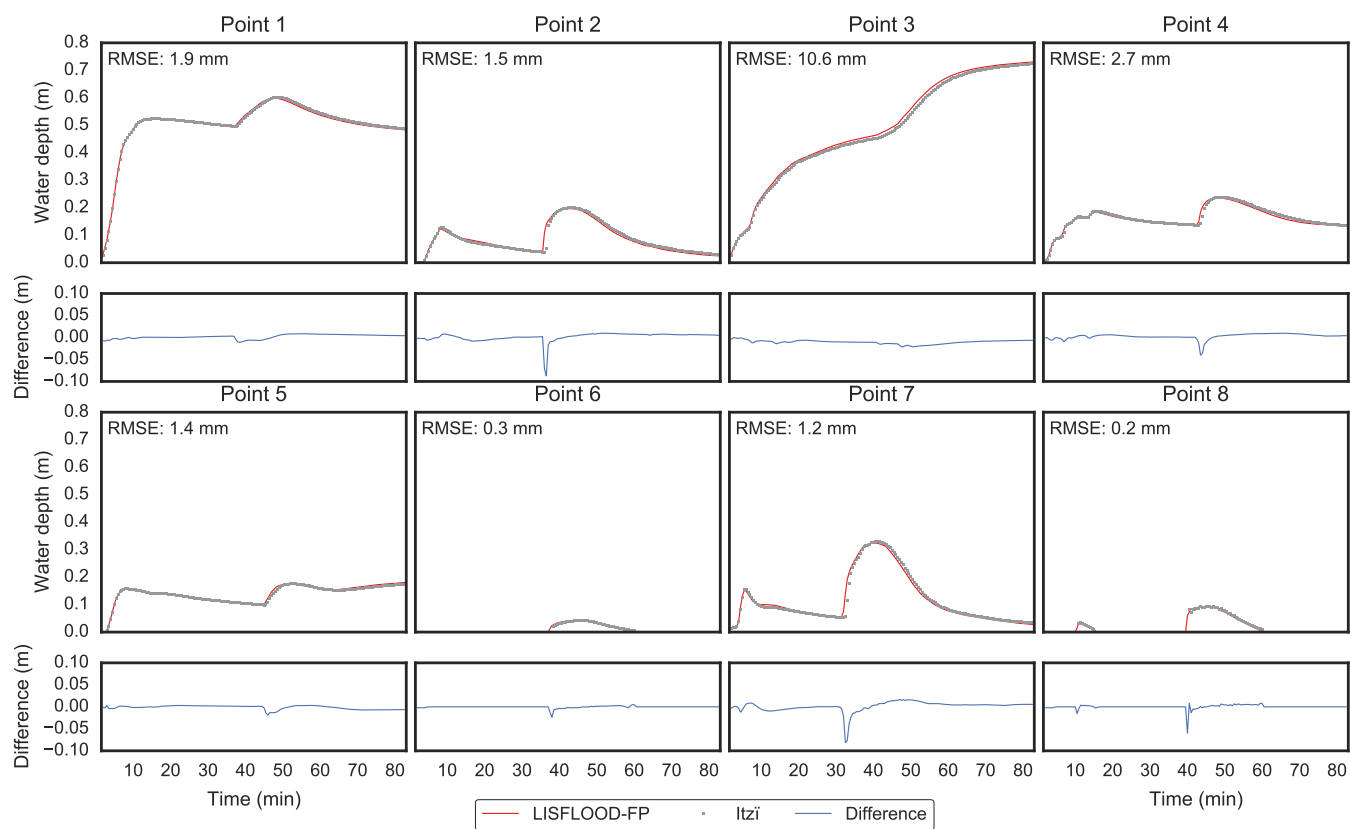
Figure 7. Comparison of water depths at control points. The blue line represents the differences of water depth between Itzi and LISLOOD-FP.
