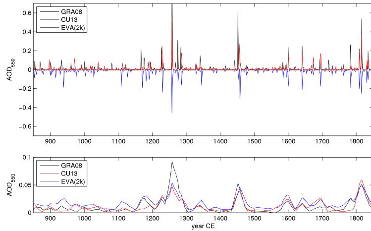
Figure 2: Reconstructions of volcanic forcing, 850-1850 CE, shown as global mean, mid-visible (550 nm) aerosol optical depth (AOD) as (top) annual means and (bottom) a smoothed time series after application of a 21-yr wide triangular filter (for visualisation). Reconstructions include the Gao et al., 2008 (GRA08), Crowley and Unterman 2013 (CU13) and the PMIP4 recommended forcing, EVA(2k). Note that the AOD in 1258 for the GRA08 reconstruction extends beyond the axis of the plot, with a value of approximately 1.05. AOD for the EVA(2k) reconstruction is shown on inverted axis in top panel for clarity.
