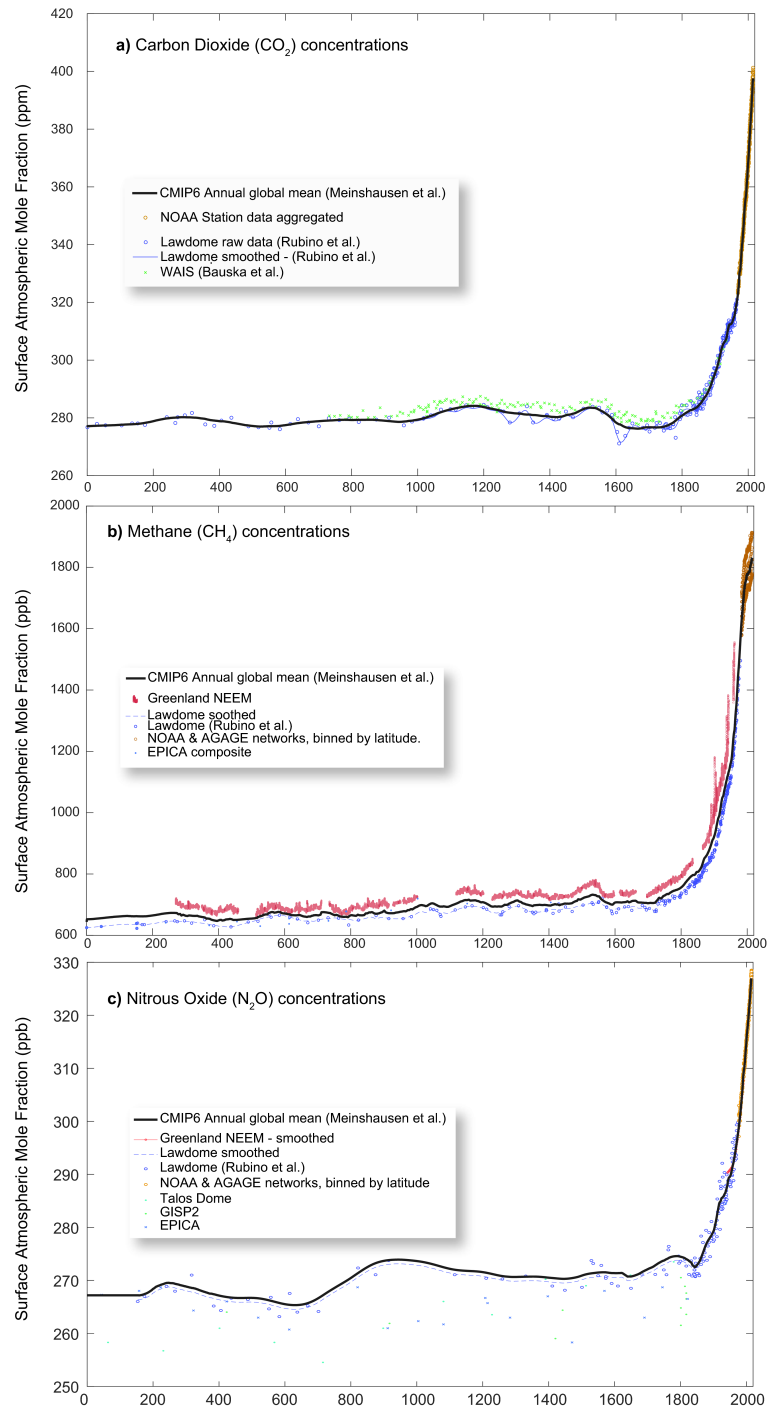
Figure 1: historical atmospheric surface concentrations from year 1BC to year 2014 CE of carbon dioxide, methane and nitrous oxide. The PMIP recommendation is to use GHG concentrations for past1000 consistent with the historical CMIP6 runs. Here shown are global-mean concentrations of these fields (thick black line), in comparison with key Antarctic ice core and Greenland firn datasets (see legend). The latitudinal gradient for \text{CO}_2 is assumed zero before 1850 CE. For methane, NEEM and Law-Dome ice core data provides an indication of the latitudinal gradient during pre-industrial times, which is reflected in the extended CMIP6 dataset. \text{N}_2\text{O} measurements from Antarctic ice cores vary substantially between studies. The extended CMIP6 dataset follows a smoothed version of the Law-Dome record.
