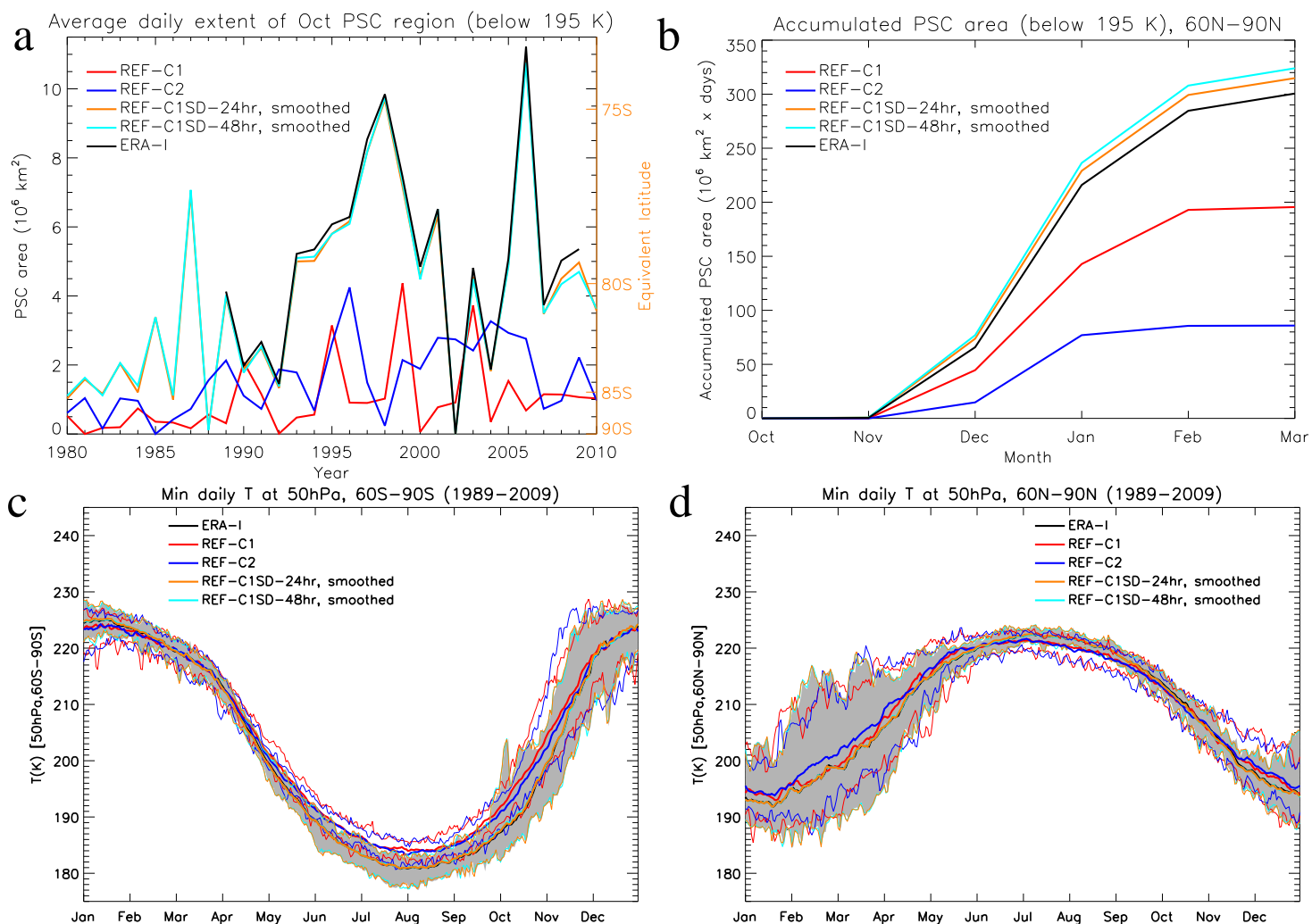
Figure 6. (a) Average daily October Nitric Acid Trihydrate (NAT) PSC area, at 50 hPa , in the southern hemisphere, defined as the area poleward of 60°S with daily mean temperatures below 195K. (b) Accumulated daily PSC area, at 50 hPa , in the northern hemisphere, defined as the area poleward of 60°N with daily mean temperature below 195K. (c) Minimum 50hPa–50 hPa daily mean temperature in the region 60°S–90°S. (d) Minimum 50hPa–50 hPa daily mean temperature in the region 60°N–90°N. Thick and thin lines, and shading, in panels (c) and (d) are as in Figure 4. All panels are averaged over years 1989–2009. Note that temperature is used as a proxy for PSC area here, and thus these are estimates of the PSC area seen by the interactive chemistry.
