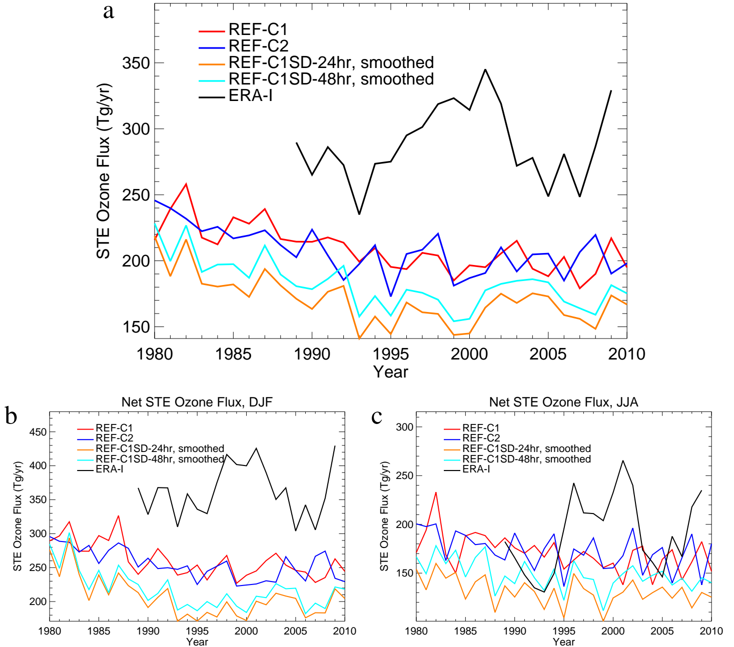
Figure 13. Stratosphere-Troposphere-Exchange of ozone for (a) annual mean, (b) December-January-February, and (c) June-July-August. This flux of ozone across the tropopause is calculated using monthly mean residual vertical velocity and ozone mass mixing ratio, following Hegglin and Shepherd (2009). The tropopause is here defined as the 100hPa 100 hPa surface equatorward of 50° and the 200hPa 200 hPa surface poleward of 50°.
