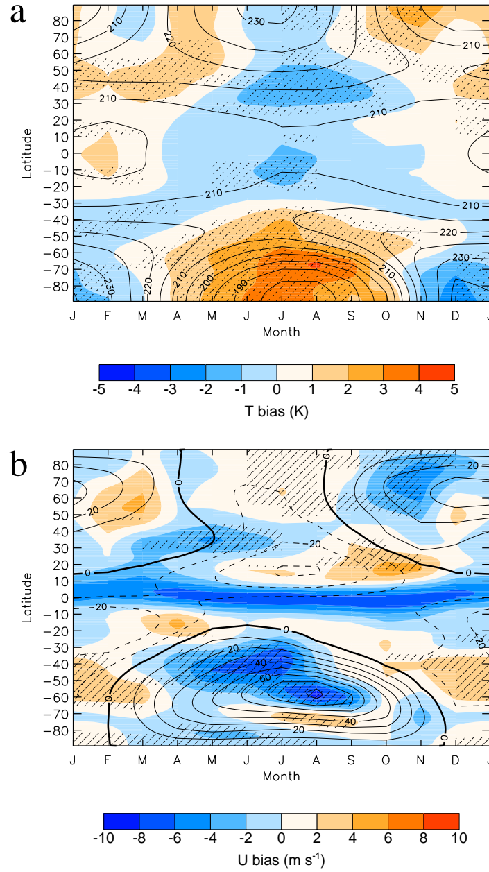
Figure 3. Biases in the climatological seasonal cycle of the REF-C1 simulation, relative to ERA-Interim, for zonal mean (a) Temperature ( 50hPa 50 hPa ) and (b) Zonal wind ( 10hPa 10 hPa ). Black contours show ERA-I values, with contour intervals of 5K and 10m 10 \text{m s}^{-1} respectively, and coloured shading shows the bias (REF-C1 minus ERA-I), with contour intervals 1K and 2m 2 \text{m s}^{-1} respectively. Stippling shows regions where the bias is statistically significant at the 95% level as calculated using a T-test. Tick marks indicate the middle of each month.
