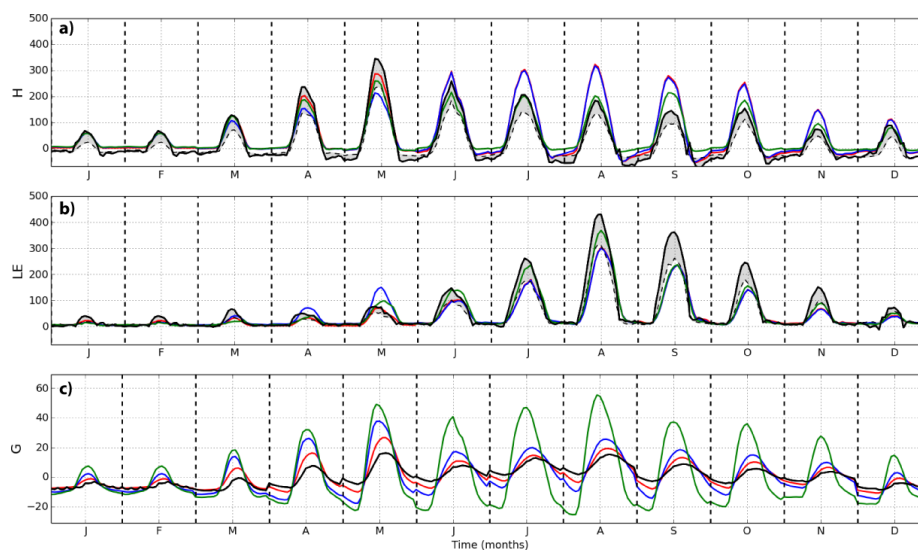
Figure 6. As in Fig.4 except for Barbeau.
