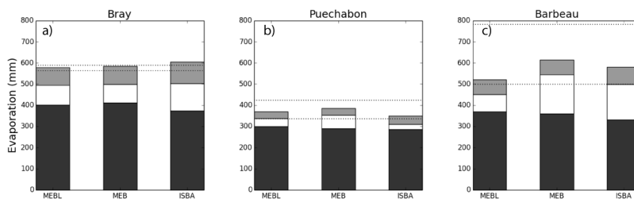
Figure 2. The partitioning of latent heat flux for each site and model option into: transpiration (black), ground/litter evaporation (white) and evaporation from the canopy (grey). Values for Le Bray, Puechabon and Barbeau are shown in panels a, b and c, respectively.
