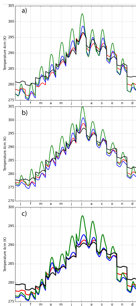
Figure 8. Monthly average soil temperature (K) diurnal cycle (at 0.04 m soil depth) composites at Le Bray (panel a), Puechabon (b) and Barbeau (c). MEBL is in red, MEB in blue, ISBA in green and the observations are shown in black.
