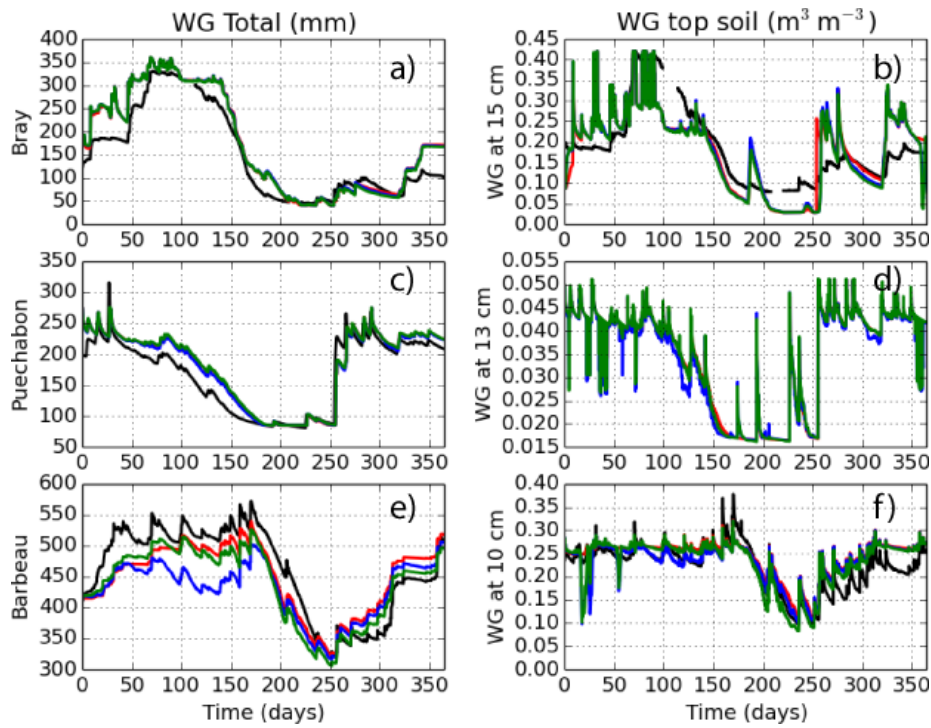
Figure 9. The total soil water content (left: panels a, c and e) and the near-surface volumetric soil water content (right: panels b, d and f) at each site. Observations are in black (for Puechabon, the black curve corresponds to the output from a site-specific calibrated reference model from Lempereur et al. (2015), see text). Results for MEBL are in red, for MEB in blue and for ISBA in green.
