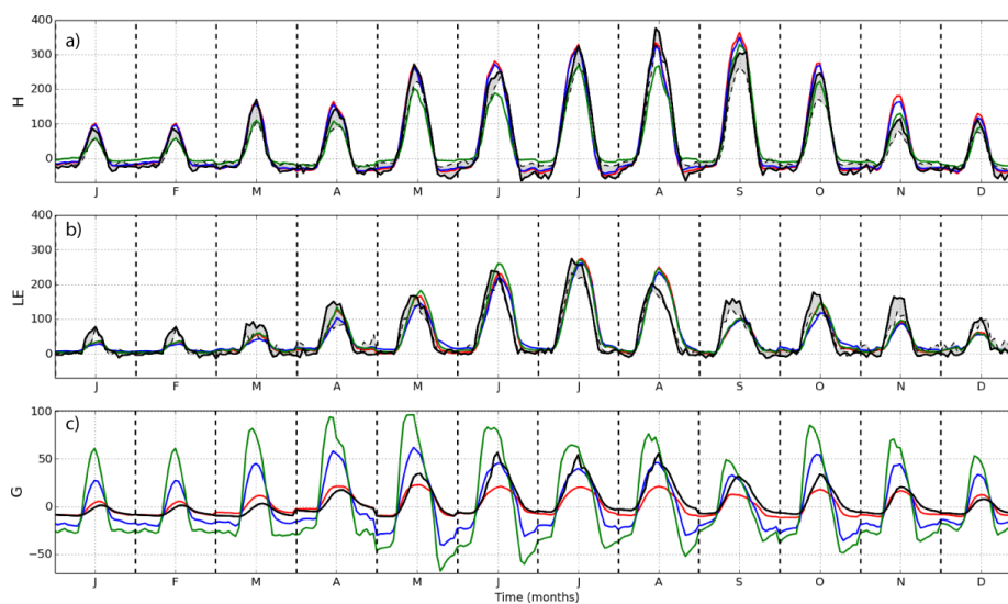
Figure 4. The monthly diurnal cycle composite at Le Bray. MEBL is in red, MEB in blue, ISBA in green, measurements are indicated by a dashed black line and adjusted measurements are represented using a solid black curve. As a visual aid, the area between the latter two curves is shaded. Ideally, model results fall within this area.
