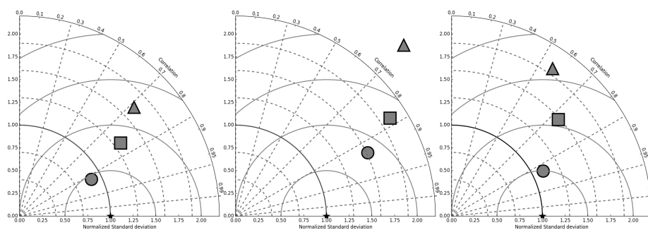
Figure 7. The Taylor diagram for ground heat flux, G , at Le Bray (panel a), Puechabon (b), and Barbeau (c). MEBL is represented by a circle, MEB by a square, ISBA by a triangle and measurements are indicated using a star. Three scores are represented in each diagram; the correlation coefficient ( R ) is the angle of the polar plot, the normalized standard deviation (NSDV) is the radial distance from the origin, and the normalized centered root mean square error (cRMSE) is proportional to the distance with the reference (star).
