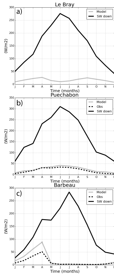
Figure 3. The modelled (thin dashed line) and observed (thick dashed line) incoming short wave radiation transmitted through the canopy at a) Le Bray, b) Puéchabon, and c) Barbeau. The observations are based on below-canopy PAR measurements. The total incoming short wave radiation is also plotted (full black line) as a reference.
