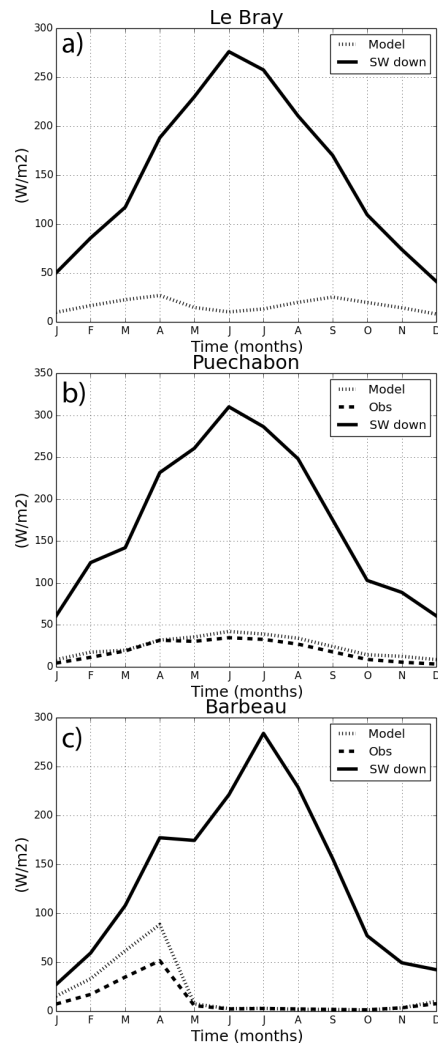
Figure 3. The modelled (thin dashed line) and observed (thick dashed line) incoming short wave radiation transmitted through the canopy at Puechabon a) Le Bray , b) Puechabon , and c) Barbeau . The observations are based on below-canopy PAR measurements. The total incoming short wave radiation is also plotted (full black line) as a reference.
