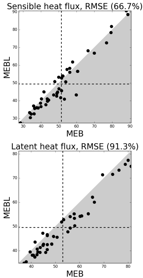
Figure C1. Scatter plots of RMSE, for sensible heat flux H (up panel) and latent heat flux LE (bottom panel) for each site and year. The abscissa corresponds to the MEB model and the ordinate to the MEBL model. Points falling within the grey shaded area imply a better statistical score for MEBL. Each dot corresponds to one site. The intersection of the dashed lines corresponds to the average over all 42 sites. The percentages at the top of each panel correspond to the percent of sites which have better statistics for MEBL.
