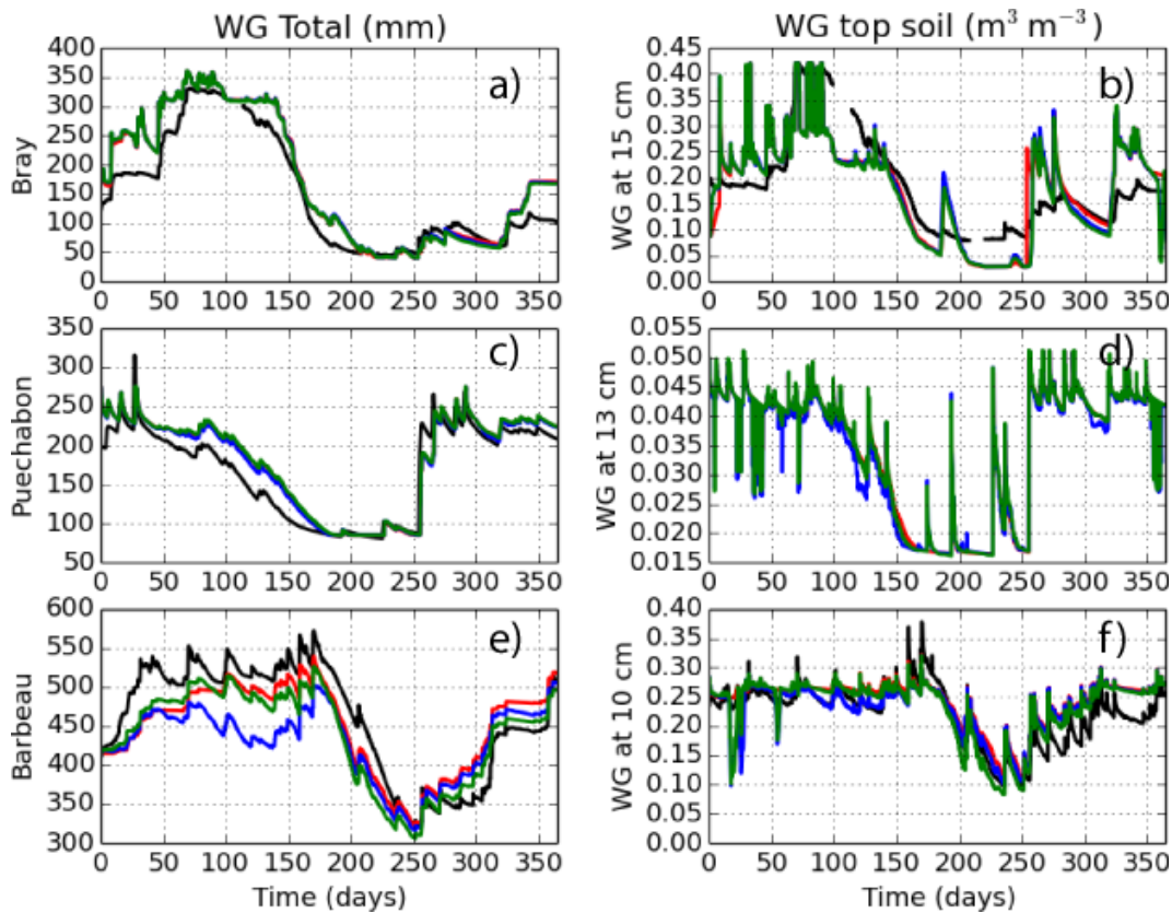
Figure 5. The total soil water content calculated over the root depth indicated in tab. Table 2 (left: panels a, c and e) and the near-surface volumetric soil water content (right: panels b, d and f) at each site. Observations are in black (for Puechabon, the black curve corresponds to the output from a site-specific calibrated reference model from Lempereur et al. (2015), see text). Results for MEBL are in red, for MEB in blue and for ISBA in green.
