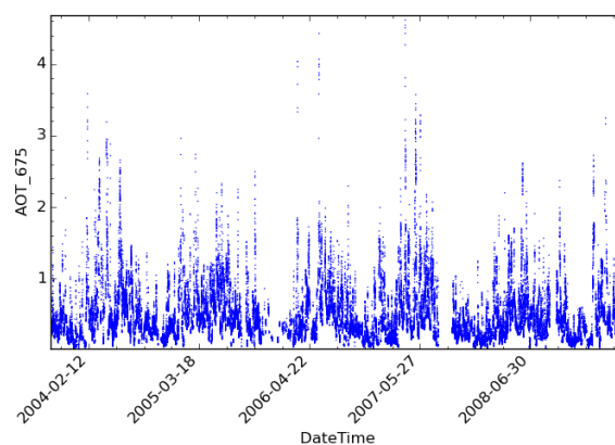
Figure 10. CIS plot with default options for AOT observed from a single AERONET station.
