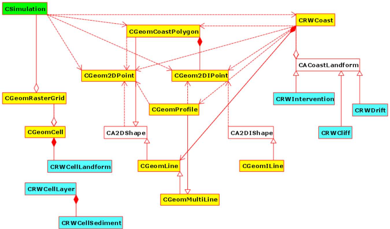
Figure 13. Class diagram showing the three main classes included in CoastalME. Classes with yellow boxes and a CGeom prefix represent geometrical objects (e.g. CGeomLine represents a line with real-valued co-ordinates, CGeomILine is the same but with integer-valued co-ordinates). Pale blue boxes and a CRW prefix denote real-world objects (e.g. CRWCliff). White boxes and a CA prefix (e.g. CA2DShape) represent abstract geometrical or real-world objects which cannot themselves be instantiated (i.e. which can only be used to construct other classes). A full list of classes and methods included in CoastalME can be found in the framwework documentation (see code availability).
