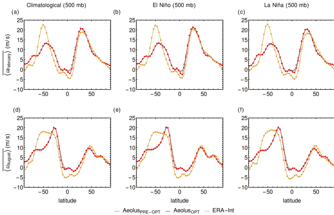
Figure 5 Zonal-mean large-scale zonal wind velocity \overline{\langle u(z, \phi) \rangle} at 500mb. (a) shows the climatological monthly mean zonal-mean zonal velocity in February, (b) depicts the monthly mean zonal-mean velocity of El Niño Februaries and (c) the monthly mean zonal-mean velocity of La Niña Februaries. (d) displays the monthly mean climatological zonal-mean zonal velocity in August, (e) shows the monthly mean zonal-mean velocity in El Niño Augusts and (f) depicts the monthly mean zonal-mean velocity in La Niña Augusts. The yellow line represents zonal-mean large-scale zonal wind obtained by reanalysis data, the gray line is zonal-mean large-scale zonal wind velocity from Aeolus using pre-optimized parameters, and the red line represents zonal-mean large-scale zonal wind velocity from Aeolus using optimized parameters.
