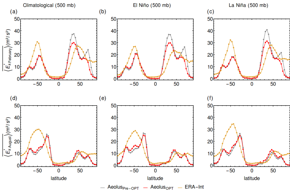
Figure 7 Zonal-mean time averaged eddy kinetic energy \overline{\langle E'_k \rangle} (compare Fig. 6).
