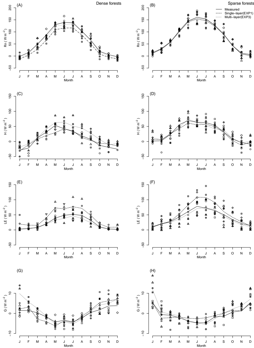
Figure 5. Inter-annual dynamic-variation of measured and simulated energy fluxes. The lines indicate mean values of selected sites (dense or sparse forests). The observed mean is shown as a solid line; and the simulations of the single-layer energy budget scheme (EXP1) and the multi-layer energy budget scheme (EXP3) are shown as a dashed and dotted line, respectively. The symbols represent the monthly averaged values of energy fluxes at one site (in the first column sub-plot A, C, E and G are dense forest sites; FI-Hyy: \square , DE-Bay: \circ , DE-Hai: \triangle and BE-Vie: \diamond ; in the second column sub-plot B, D, F and H are sparse forest sites; FR-LBr: \square , NL-Loo: \circ , CA-Oas: \triangle and AU-Tum: \diamond ). Simulation results are symbols filled with colors, EXP1 with gray color and EXP3 with black color.
