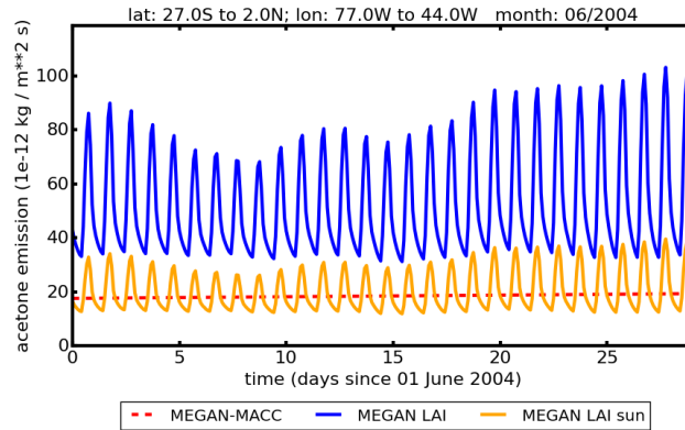
Figure 7. Acetone emission comparison of MEGAN-MACC (red dashed), MEGAN-Online LAI (blue) and MEGAN-Online LAI_{sun} (orange) averaged over South America ( 77 to 44^\circ W and 27^\circ S to 2^\circ N) in June 2004.
