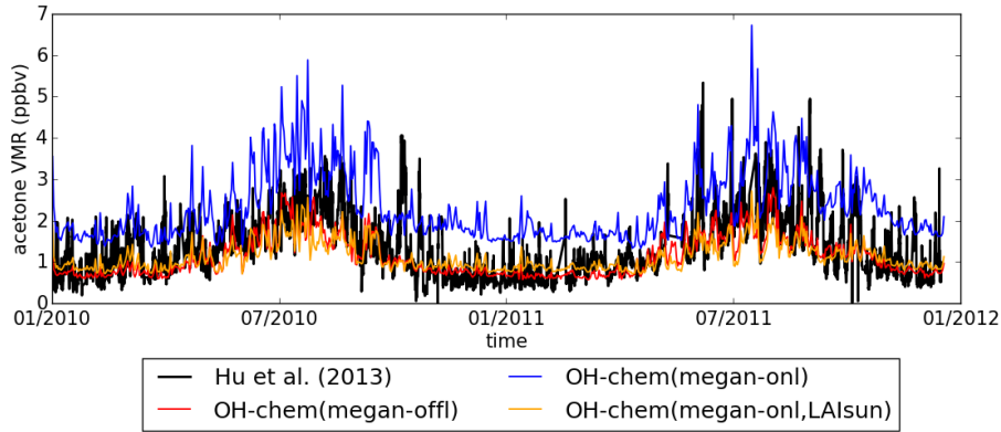
Figure 10. Measured (black) and simulated (red: OH-chem(megan-offl), blue: OH-chem(megan-onl), orange: OH-chem(megan-onl,LAIsun)) acetone VMR interpolated to the observation site in Minnesota (USA), see Hu et al. (2013). The measurement error of 10 % is not included in the figure.
