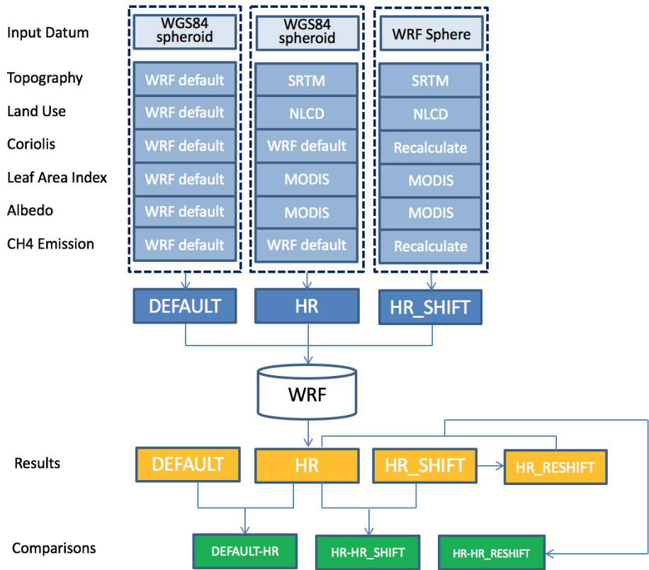
Figure 5. Workflow of the study showing the three scenarios: DEFAULT, HR, HR_SHIFT.
