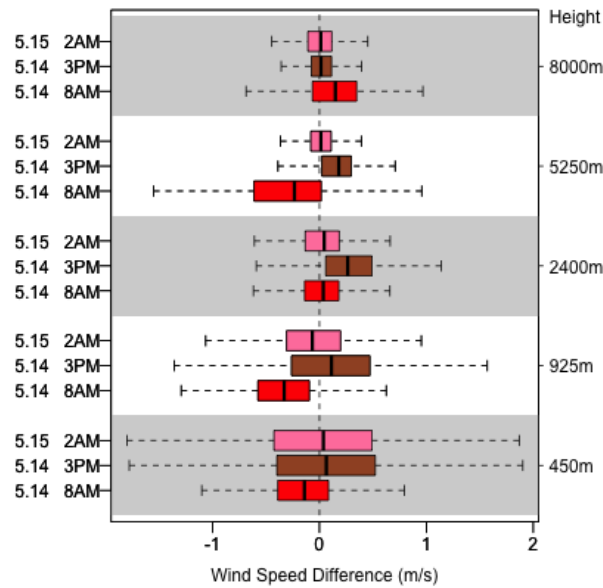
Figure 15. Wind speed differences between HR and HR_RESIFT in the domain 3.
