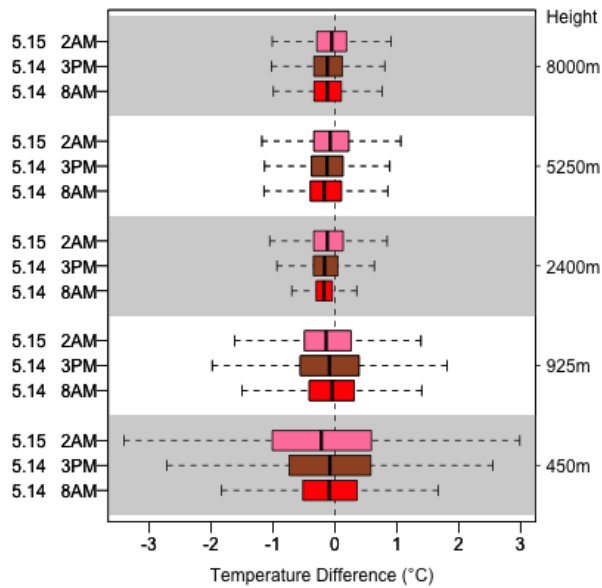
Figure 11. Temperature differences between HR and DEFAULT_HR_RESHIFT in the domain 3.2. Wind-speed differences between HR and DEFAULT in the domain 3.
