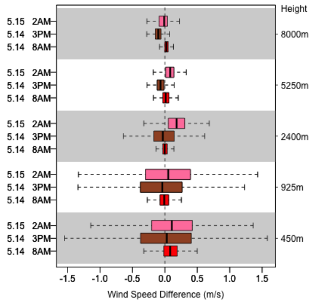
Figure 9. Wind speed differences between HR and DEFAULT in the domain 3.
