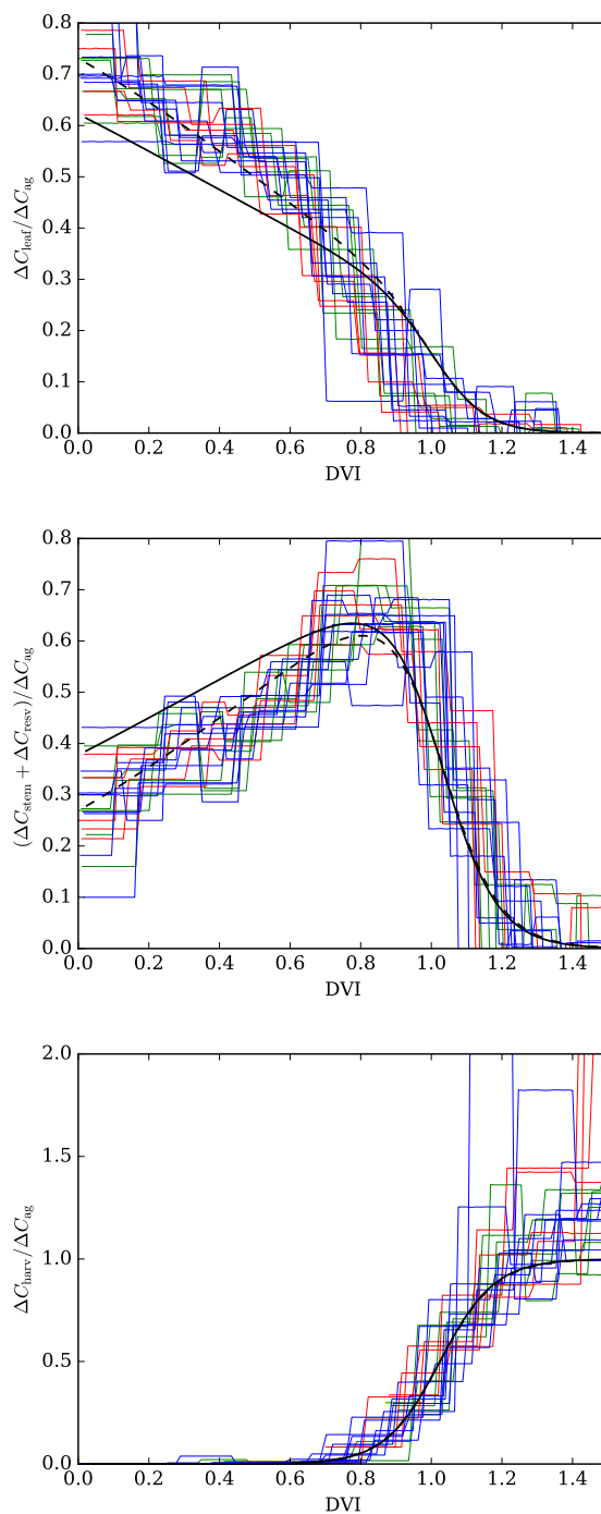
Figure 1. Top: ratio of rate of change of C_{leaf} to rate of change of above-ground carbon C_{ag} , middle: ratio of rate of change of C_{stem} + C_{resv} to rate of change of above-ground carbon, bottom: ratio of rate of change of C_{harv} to rate of change of above-ground carbon. Solid black line uses the original crop parameters from Osborne et al. (2015), dashed black line uses the tuned parameters. Blue, green, red lines are derived from US-Ne1, US-Ne2 and US-Ne3 observations respectively.
