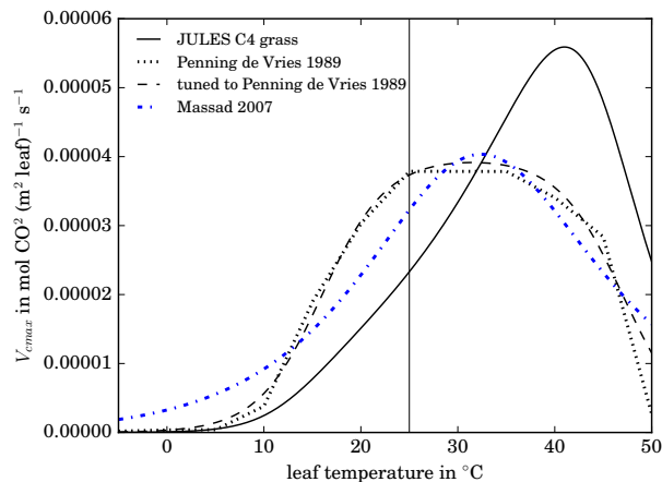
Figure 17. Parametrisations of V_{cmax} against leaf temperature. Solid black line shows default C4 grass in JULES. Dotted line shows the parameterisation for maize given in de Vries et al. (1989), black dashed line shows a fit to this using the JULES parameterisation. Blue dot-dashed shows the parameterisation for maize in Massad et al. (2007).
