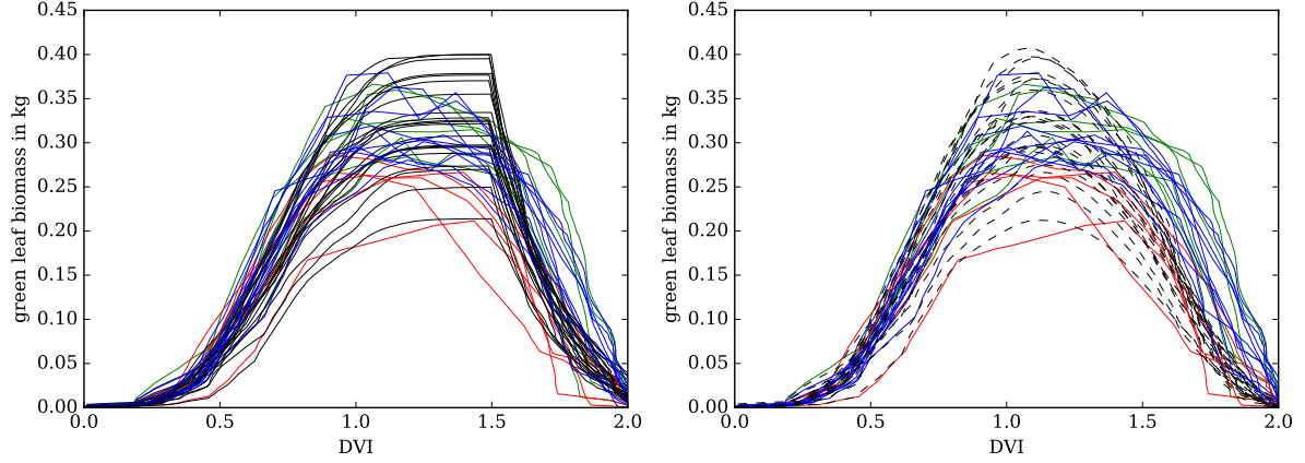
Figure 4. Green leaf biomass against DVI. Blue, green, red lines are derived from US-Ne1, US-Ne2 and US-Ne3 observations respectively. Black lines are generated using model parameters from Osborne et al. (2015) (left plot, solid lines) and the new, tuned parameters (right plot, dashed lines).
