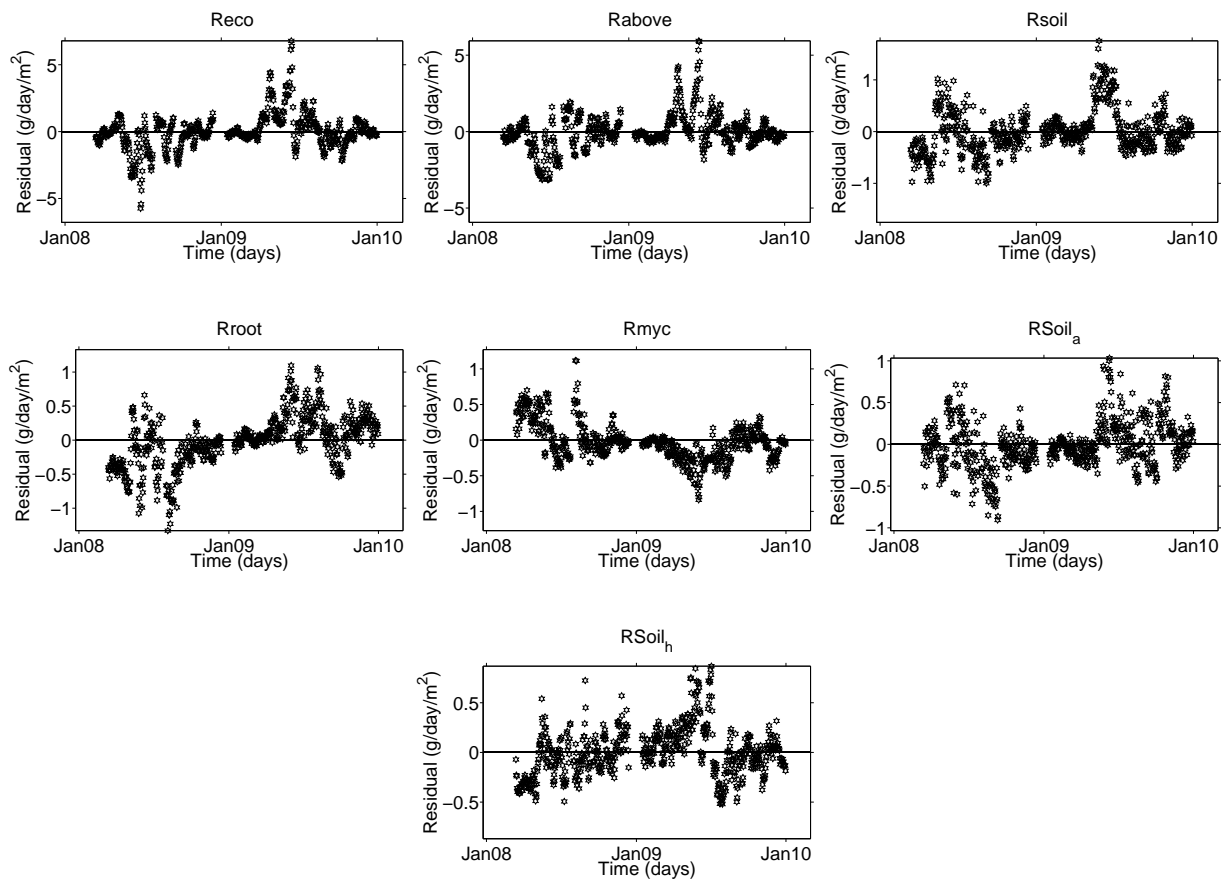
Figure 11. Residuals computed for smear term bias corrected back-transformed GEP models for various types of \text{CO}_2 respiration fluxes after training against log-transformed targets with the settings given in column 2 of Tab. 1.
