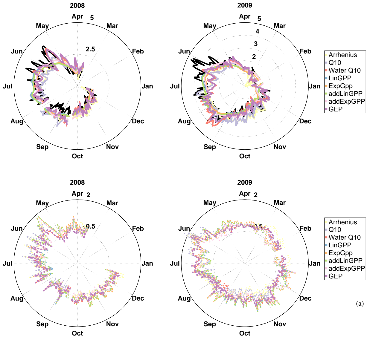
Figure 15. Daily R_{soil} fluxes (A) illustrated in the context of the two studied years and residual values (B) of the total soil daily CO_2 outgoing fluxes as simulated by the investigated literature models and the GEP emerged model after smear term bias corrected back-transformation. The fluxes shown here are the real flux measured at the site and the predicted fluxes generated according to the GEP model and some of the models used in the environmental science community. The centre of the plots in the second row is -1. The scale of the fluxes is given in gC/m^2/day .
