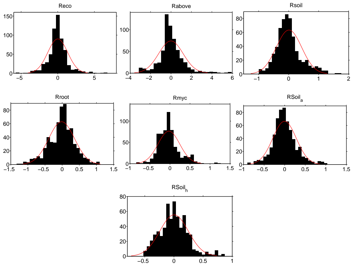
Figure 3. Distributions of the residuals after smear bias correction computed for the GEP models after training on log-transformed data.
