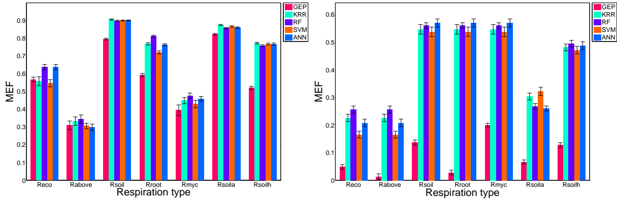
Figure 13. Machine learning methods (MLM) prediction performance for all respirations components (left) and for the residuals (right) resulting from the GEP trained models after smear term bias corrected back-transformation. The MEF values obtained for validation by all the MLM methods for R_{eco} , R_{above} , R_{soil} , R_{root} , R_{myc} , R_{soil_a} , R_{soil_h}
