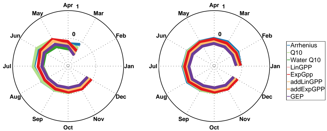
Figure 4. Monthly averaged error values for some literature models for and the GEP generated model for daily soil CO 2 efflux in the two studied years. The centre of the plots is -1. The scale of the fluxes is given in gC/m 2 /day.
