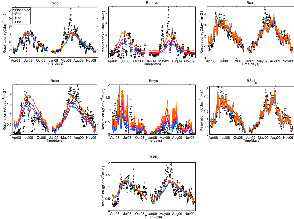
Figure 7. Observed and predicted outgoing CO 2 fluxes. 613 time steps of daily averaged CO 2 effluxes for two years at the Alice Holt oak forest site. The predicted values are generated with the models extracted by the GEP approach with the settings given in table 1 for the following types of respiration: R_{eco} , R_{above} , R_{soil} , R_{root} , R_{myc} , R_{soil_a} , R_{soil_h} and back-transformed with 3 types of residual bias correction terms: smear term, naive, and log normal term.
