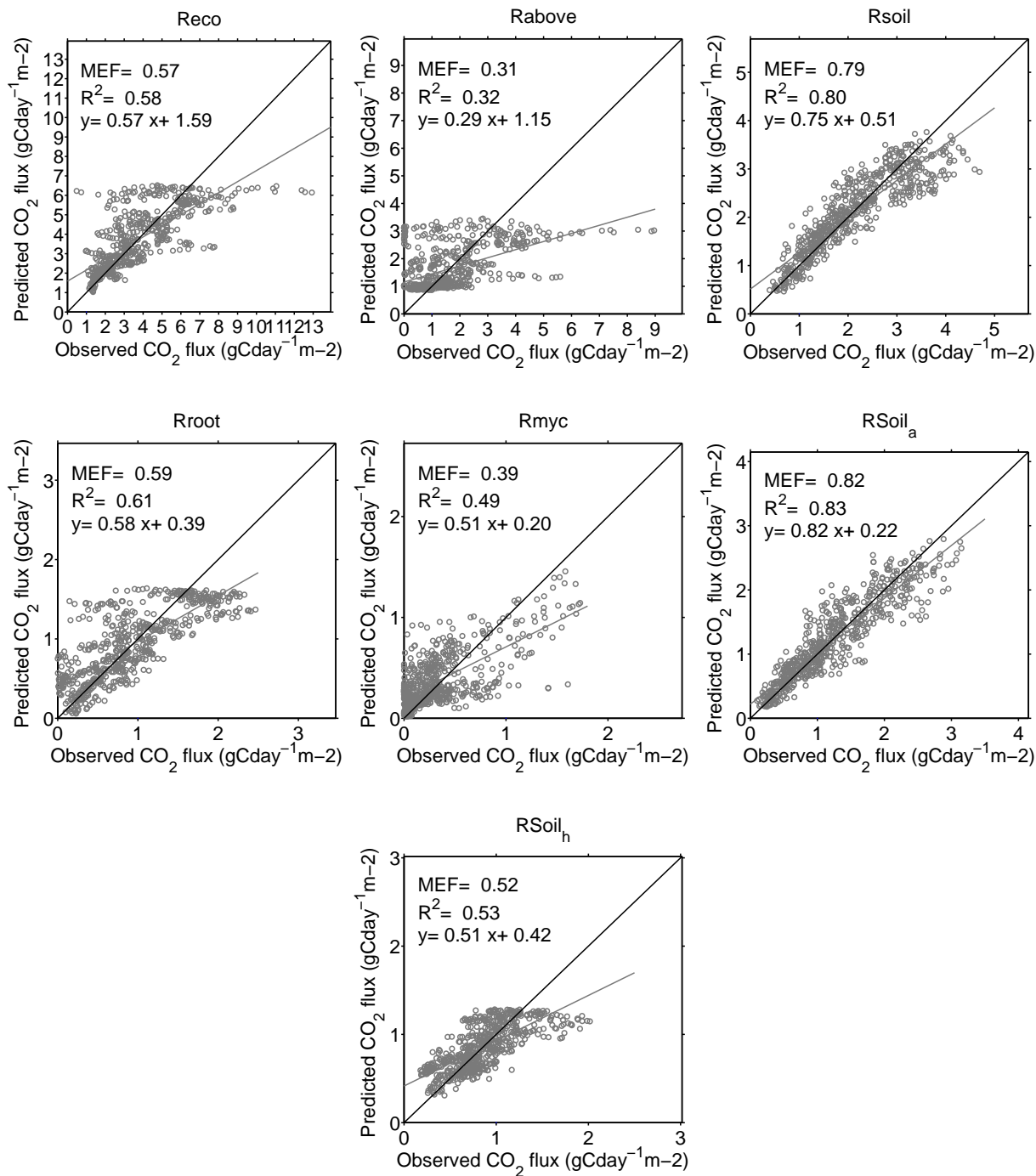
Figure 8. Observed and predicted outgoing CO 2 fluxes. 613 time steps of daily averaged CO 2 effluxes for two years at the Alice Holt oak forest site. The predicted values are generated with the models extracted by the GEP approach with the settings given in table 1 for the following types of respiration: R_{eco} , R_{above} , R_{soil} , R_{root} , R_{myc} , R_{soil_a} , R_{soil_h} and back-transformed with a smear term bias correction. The models are given in equations: 4.2-4.8
