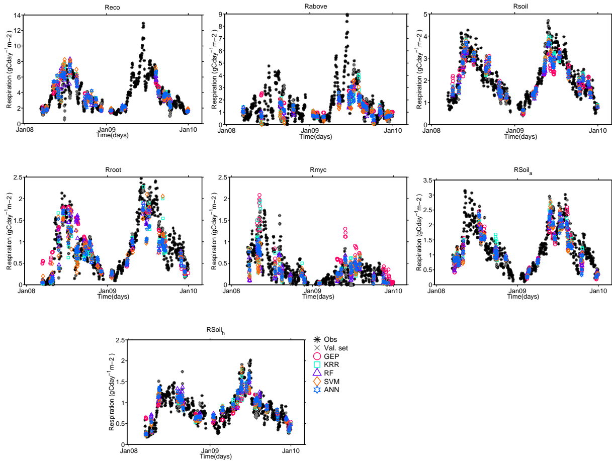
Figure 12. Observed CO_2 fluxes and one set of 113 predicted values given by the some common machine learning methods (MLM) after training on 500 data points after smear term bias corrected back-transformation.
