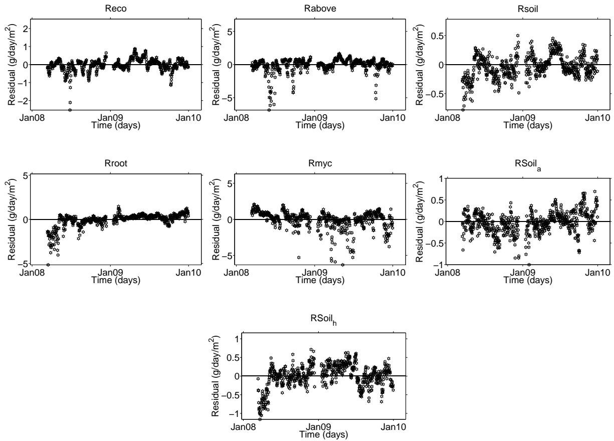
Figure 2. Residuals computed for the GEP models against the log-transformed targets before back-transformation.
