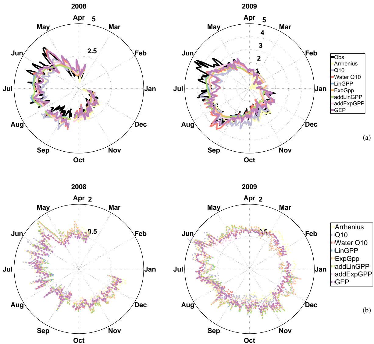
Figure 13. Daily R_{soil} fluxes (A) illustrated in the context of the two studied years and residual values (B) of the total soil daily CO 2 outgoing fluxes as simulated by the investigated literature models and the GEP emerged model. The fluxes shown here are the real flux measured at the site and the predicted fluxes generated according to the GEP model and some of the models used in the environmental science community. The center of the plots in the second row is -1. The scale of the fluxes is given in gC/m 2 /day.
