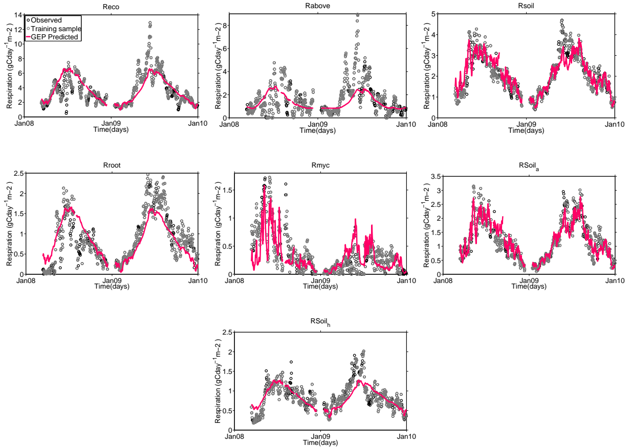
Figure 6. Observed and predicted outgoing CO 2 fluxes. 613 time steps of daily averaged CO 2 effluxes for two years at the Alice Holt oak forest site. The predicted values are generated with the models extracted by the GEP approach with the settings given in table 1 for the following types of respiration: R_{eco} , R_{above} , R_{soil} , R_{root} , R_{myc} , R_{soil_a} , R_{soil_h} . The models are given in equations: 4.2-4.8
