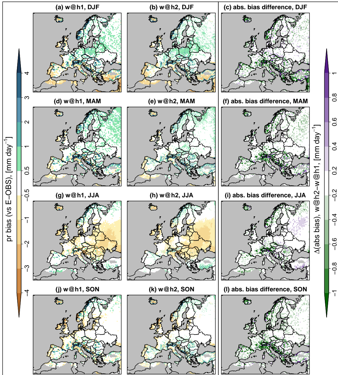
Figure 8. Same as Fig. 6 but for precipitation, in \text{mm day}^{-1} . See Supplementary Fig. S13 for these biases in relative terms.
