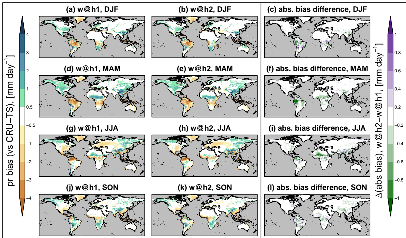
Figure 3. Same as Fig. 2 but for precipitation, in \text{mm day}^{-1} .
