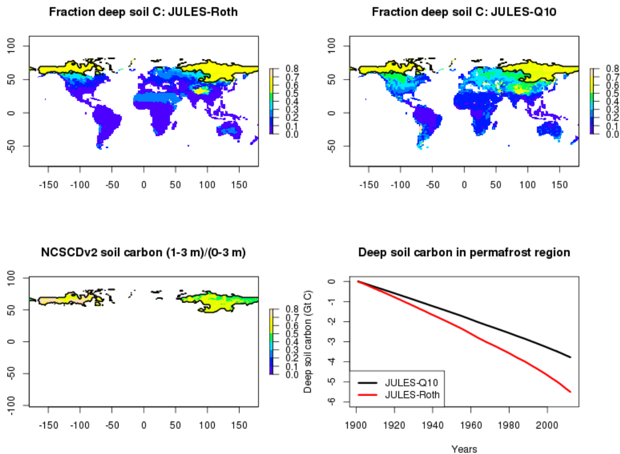
Figure 11. The spatial plots show the deep soil carbon (defined as soil carbon below 1 m in 1901) as a fraction of the total soil carbon for each grid cell. The time series shows the change in labelled deep soil carbon for the permafrost region in Pg C.
