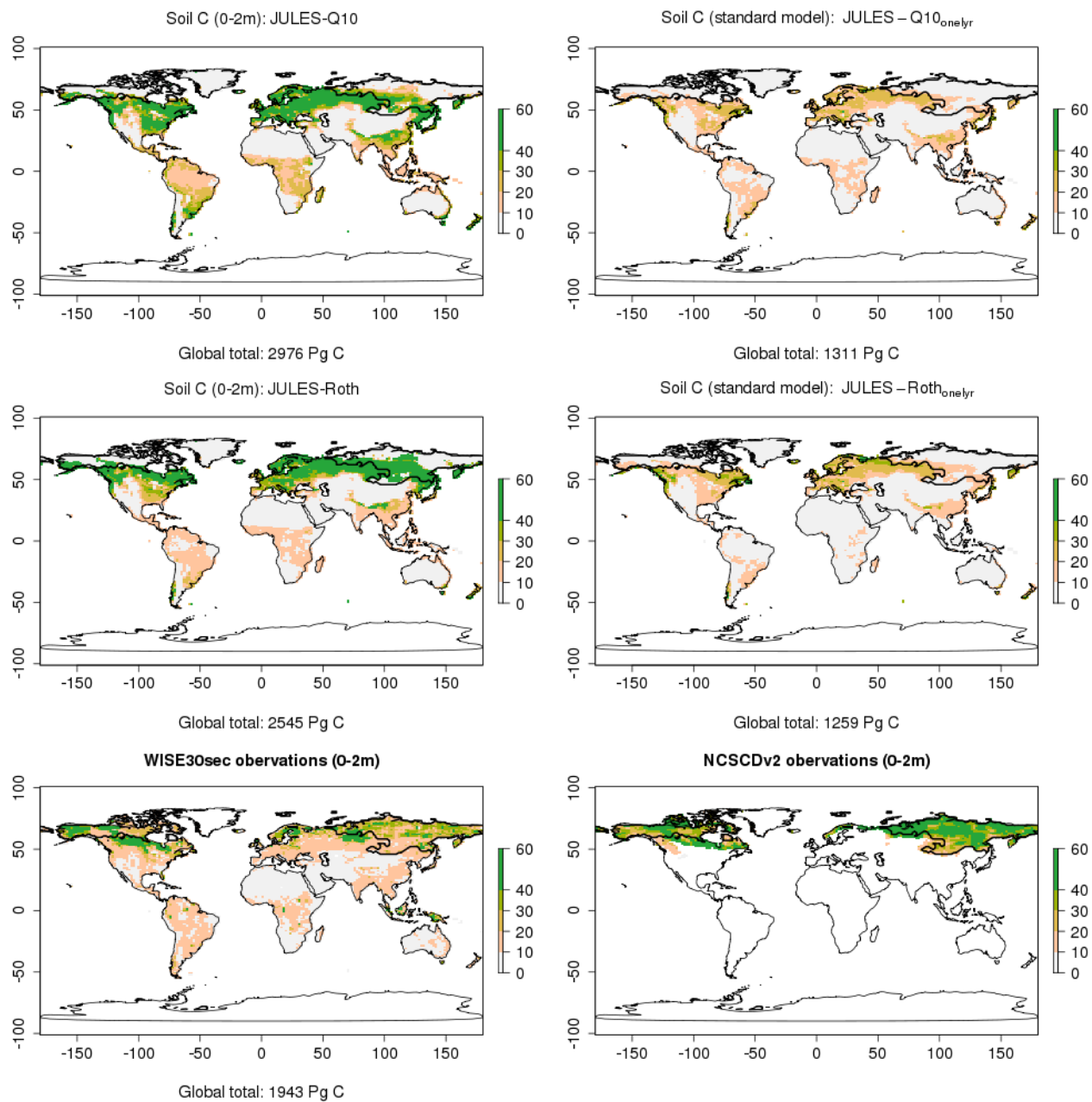
Figure 5. Soil carbon in the top 2 m in \text{kg m}^{-2} for the 4 different model simulations. The new vertically discretised model versions are on the left and the standard model versions are on the right. The WISE30sec observed data set is shown at the bottom left and the NCSCDv2 at the bottom right .
