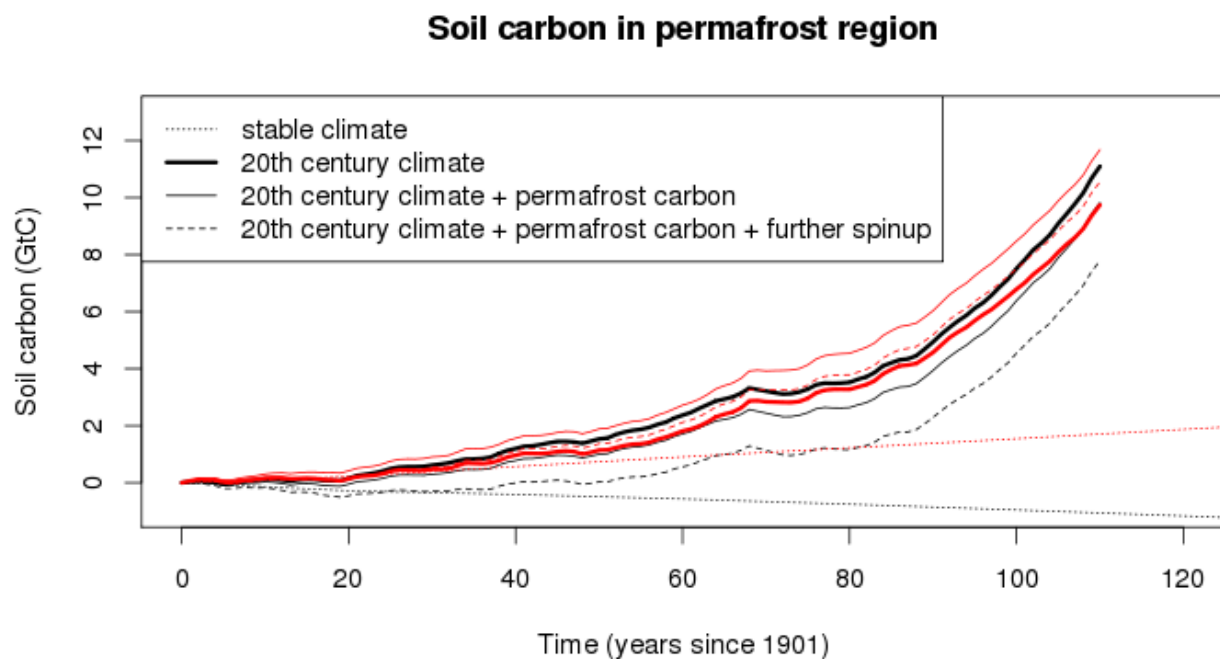
Figure 13. Change in soil carbon over 20 th century with and without the observed permafrost carbon added, and with and without further spin-up.
