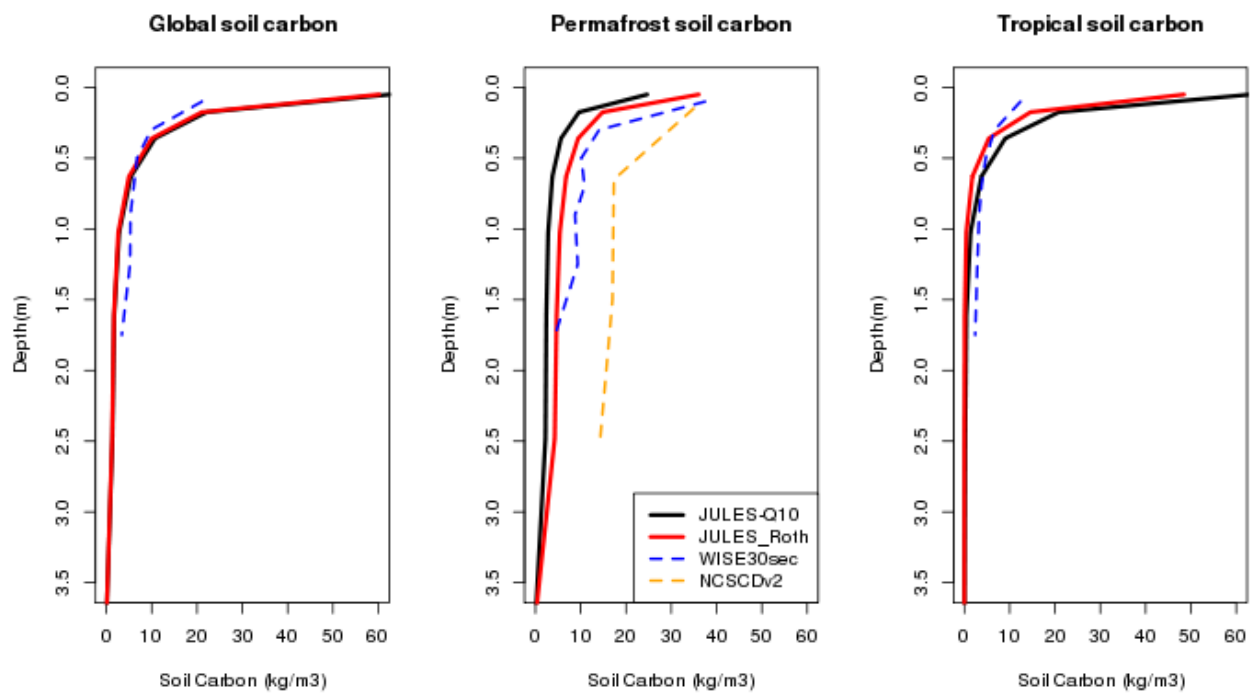
Figure 7. Profile of soil carbon in kg m -3 for the three main regions in this study.
