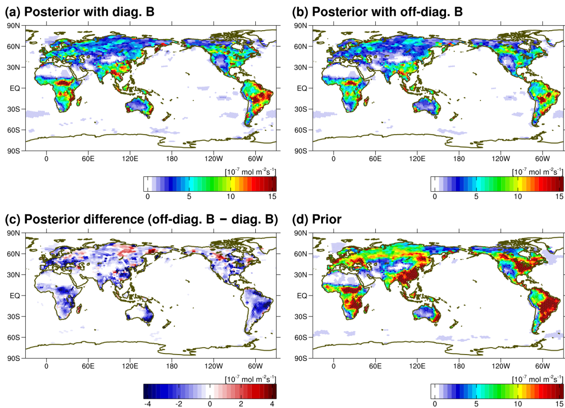
Figure 5. Root-mean-square error (RMSE) distributions of the posterior fluxes derived by POPULAR+ NON-LINEAR NONLINEAR with the diagonal B (a) and the off-diagonal B (b). The difference between (b) and (a) is shown in (c) as well as the RMSE distribution of the prior flux (d).
