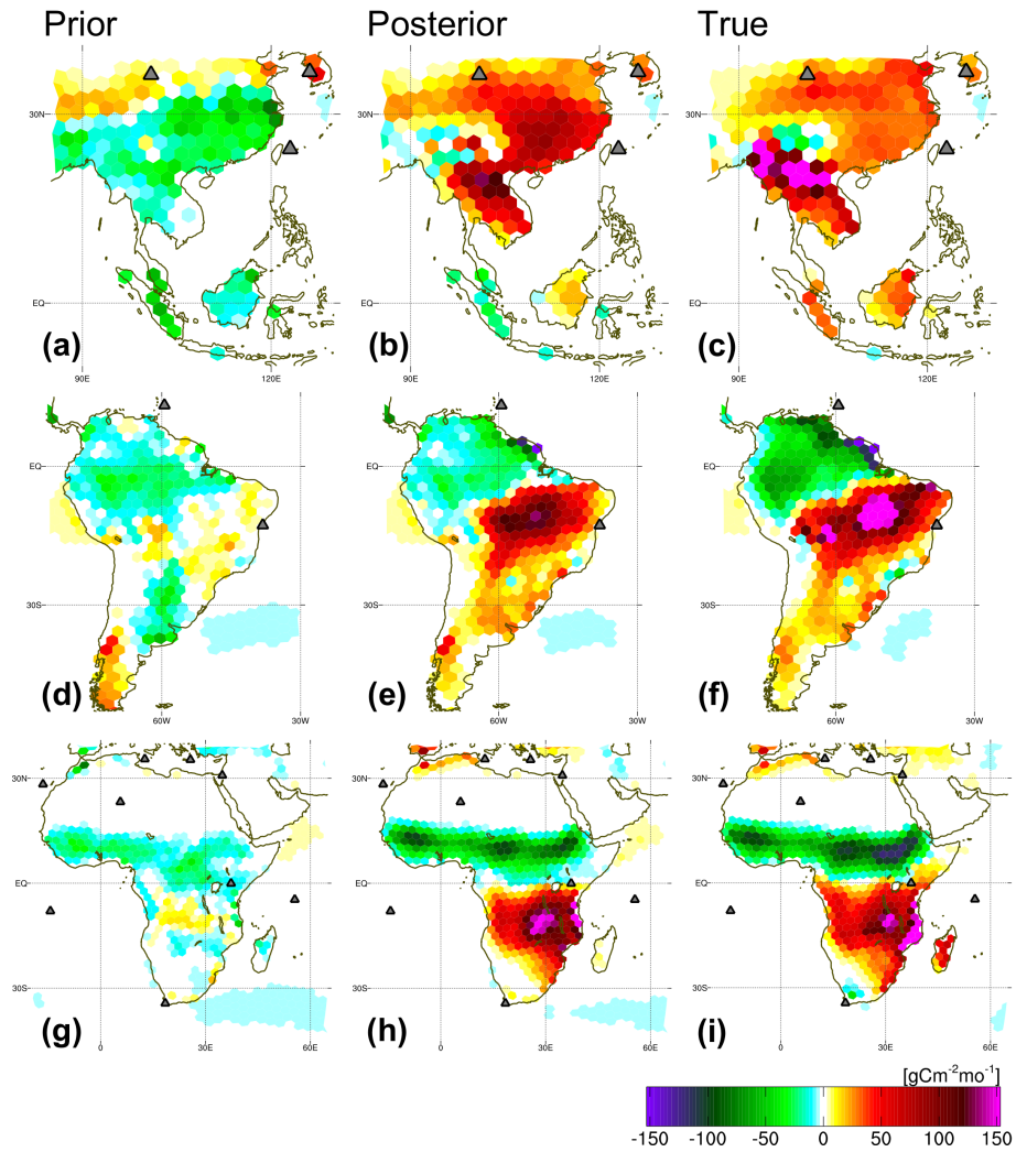
Figure 8. Same as Fig. 67, but focused on regional flux anomalies due to biomass burnings for Southeast Asia in March (a-c), South America in September (d-f), and Africa in September (g-i). Gray triangles denote locations of the observational sites.
