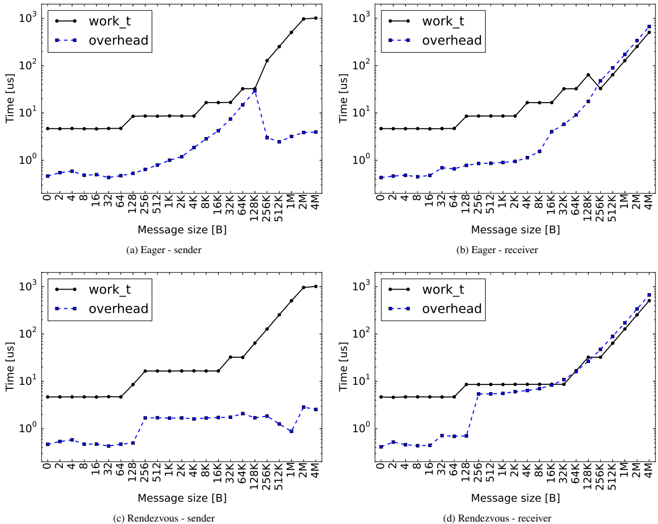
Figure 1. Results from the Sandia MPI MicroBenchmark using the IBM MPI implementation with Eager protocol (top) for sending (a) and receiving (b) an asynchronous non-blocking message and Rendezvous protocol (bottom) for sending (c) and receiving (d). Here, overhead corresponds to the amount of overhead time required to send or receive a non-blocking message, while work_t corresponds to the amount of computation required to effectively hide the costs of sending or receiving the message.
