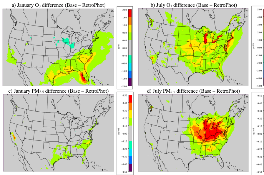
Figure 3. Difference in the monthly average O 3 for a) January and b) July and PM 2.5 for c) January and d) July between CMAQ v5.1_base and v5.1_RetroPhot (v5.1_Base - v5.1_RetroPhot). O 3 plots are in units of \text{ppbV} and PM 2.5 plots are in units of \mu\text{gm}^{-3} . Note that the scales for between each plot can vary.
