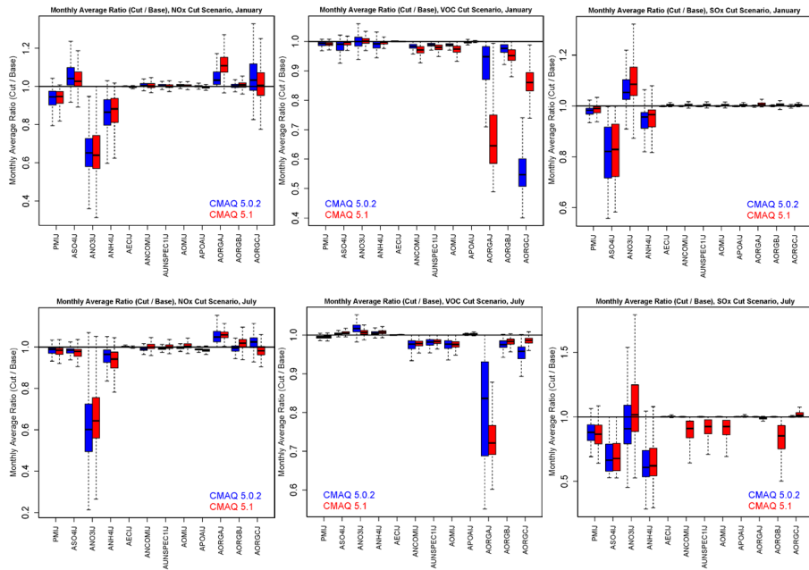
Figure 18. Box plots of monthly average ratio values (Cut /Base) of PM 1 (total PM 2.5 ), ASO 4 I, ANO 3 I, ANH 4 I, AECI, ANCOMI, AUNSPECI, AOMI, APOAI, AORGAJ, AORGBI, and AORGCJ for v5.0.2 (blue) and v5.1 (red) for a 50% cut in anthropogenic NO x (left), VOC (middle) and SO x (right) for January (top) and July (bottom).
