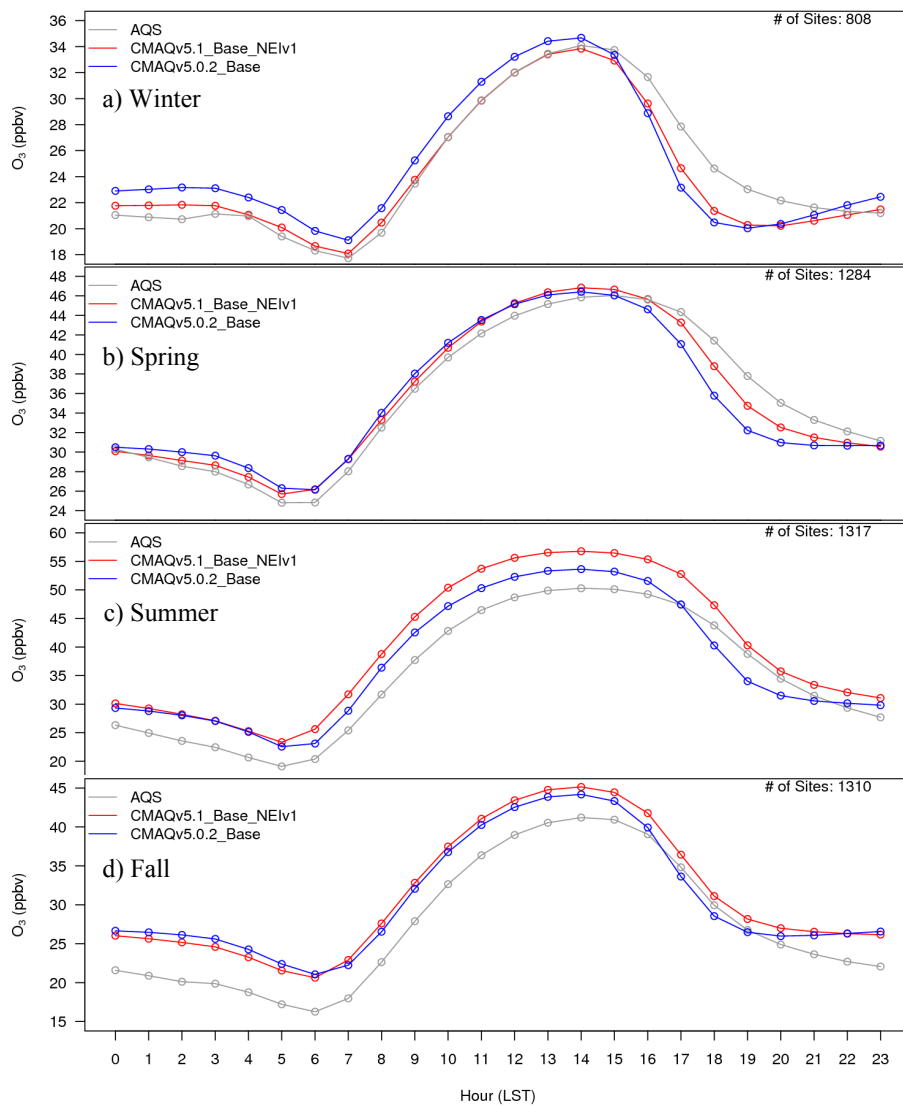
Figure 14. Diurnal time series of seasonal O_3 (ppbv) from for AQS observations (grey), CMAQv5.0.2_Base simulation (blue) and CMAQv5.1_Base_NEIv1 simulation (red) for a) winter b) spring c) summer and d) fall.
