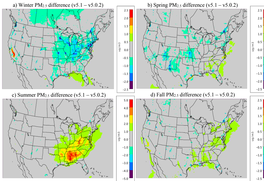
Figure 6. Difference in the seasonal average PM_{2.5} for a) winter (DJF) b) spring (MAM) c) summer (JJA) and d) fall (SON) between CMAQv5.0.2_Base and CMAQv5.1_Base NEIv1 (CMAQv5.1_Base NEIv1 - CMAQv5.0.2_Base). All plots are in units of \mu\text{gm}^{-3} .
