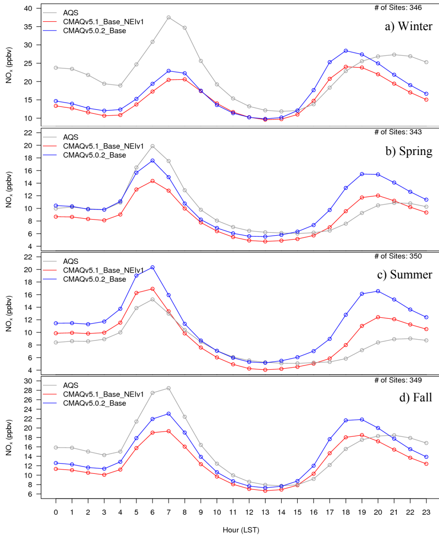
Figure 15. Diurnal time series of seasonal NO x (ppbv) from for AQS observations (grey), CMAQv5.0.2_Base simulation (blue) and CMAQv5.1_Base_NEIv1 simulation (red) for a) winter b) spring c) summer and d) fall.
