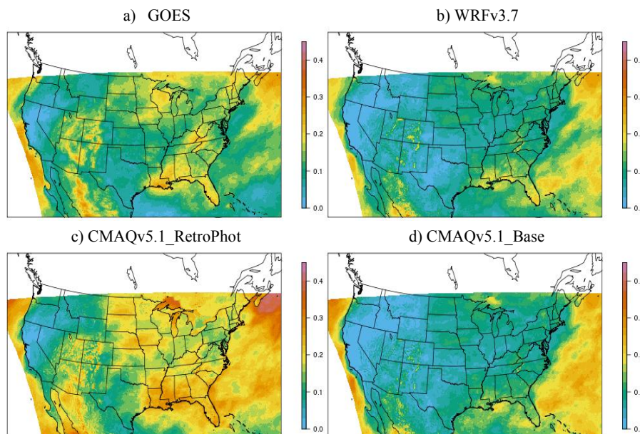
Figure 4. The average cloud albedo during daytime hours in July 2011 with available satellite data ( n = 301 hours total) derived from (a) the GOES satellite product (b) WRF3.7 (c) CMAQv5.1 with photolysis/cloud model treatment from v5.0.2 and WRF3.7 inputs (CMAQv5.1_RetroPhot) (d) CMAQv5.1 using WRF3.7 inputs (CMAQv5.1_Base_NEIv2).
