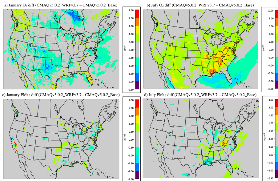
Figure 1. Monthly average difference in O_3 - O_3 ( ppbV - ppbV ) for a) January and b) July and PM_{2.5} - PM_{2.5} ( \mu g m^{-3} - \mu g m^{-3} ) for c) January and d) July between CMAQv5.0.2 using WRFv3.4 (CMAQv5.0.2_Base) and CMAQv5.0.2 using WRFv3.7 (CMAQv5.0.2_WRFv3.7) (CMAQv5.0.2_WRFv3.7 - CMAQv5.0.2_Base). Note that the scales for between each plot can vary.
