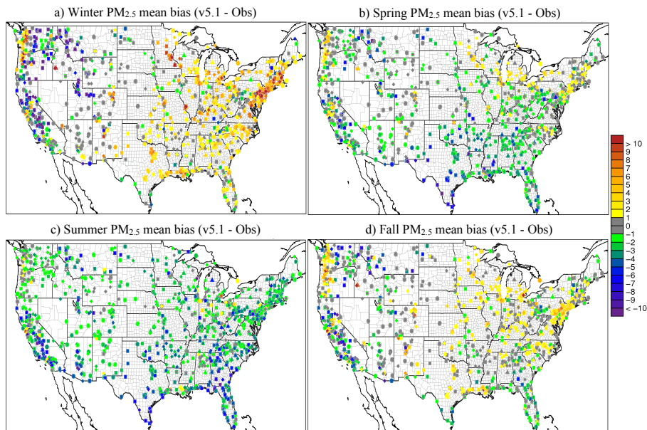
Figure 7. Seasonal average PM_{2.5} mean bias ( \mu\text{gm}^{-3} ) at IMPROVE (circles), CSN (triangles), AQS Hourly (squares) and AQS Daily (diamonds) sites for a) winter (DJF) b) spring (MAM) c) summer (JJA) and d) fall (SON) for the CMAQ v5.1_Base simulation.
