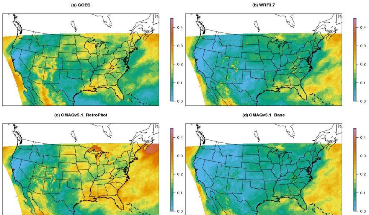
Original Figure 4 (with new color legend showing albedo as a fraction rather than a percent): The average cloud albedo during daytime hours in July 2011 derived from (a) the GOES satellite product (b) WRF3.7 (c) CMAQv5.1 with photolysis/cloud model treatment from v5.0.2 and WRF3.7 inputs (CMAQv5.1_RetroPhot) (d) CMAQv5.1 using WRF3.7 inputs (CMAQv5.1_Base).
