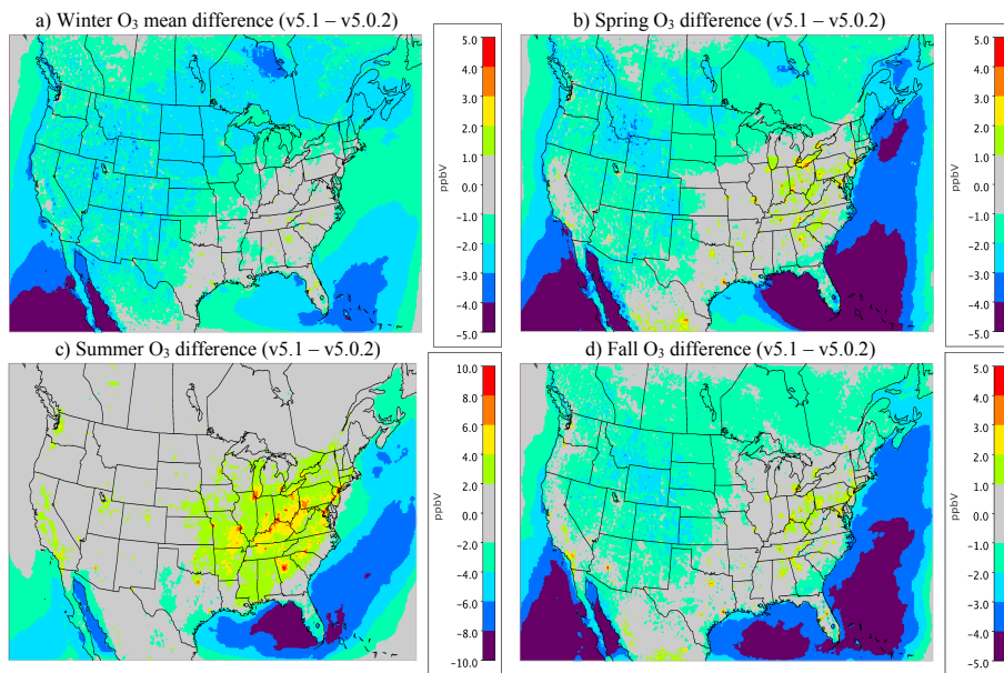
Figure 11. Difference in the monthly average hourly O_3 ( \text{ppbVppbv} ) for winter (DJF; top left), spring (MAM; top right), summer (JJA; bottom left) and fall (SON; bottom right) between CMAQ v5.0.2_Base and v5.1_Base_NEIv1 (CMAQv5.1_Base_NEIv1 - CMAQv5.0.2_Base). Note that the scales for between each plot can may vary.
