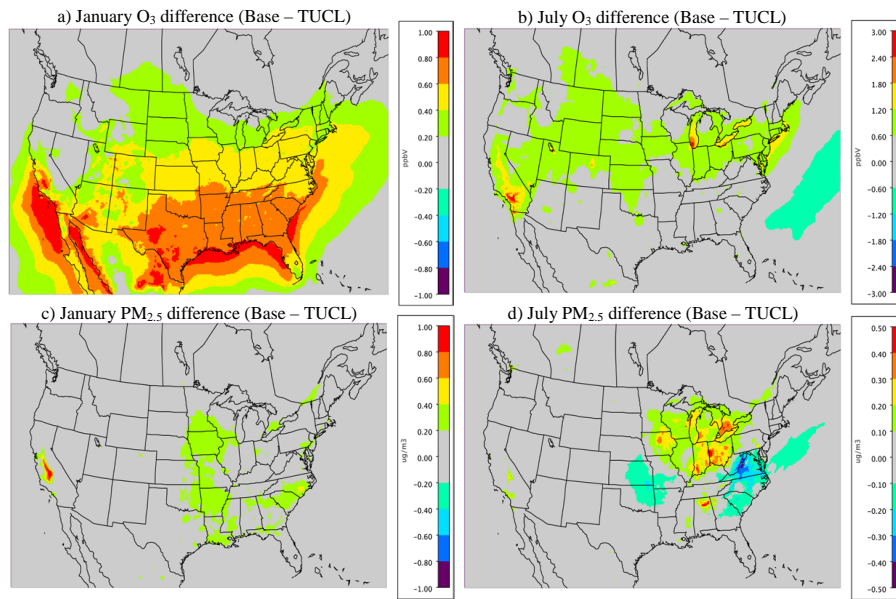
Figure 5. Difference in the monthly average O_3 for a) January and b) July and PM_{2.5} (with organic matter mass removed) for c) January and d) July between CMAQ v5.1_Base NEIv2 and v5.1_TUCL (CMAQv5.1_Base NEIv2 - CMAQv5.1_TUCL). O_3 plots are in units of ppbv and PM_{2.5} plots are in units of \mu\text{gm}^{-3} . Note that the scales for each plot can vary.
