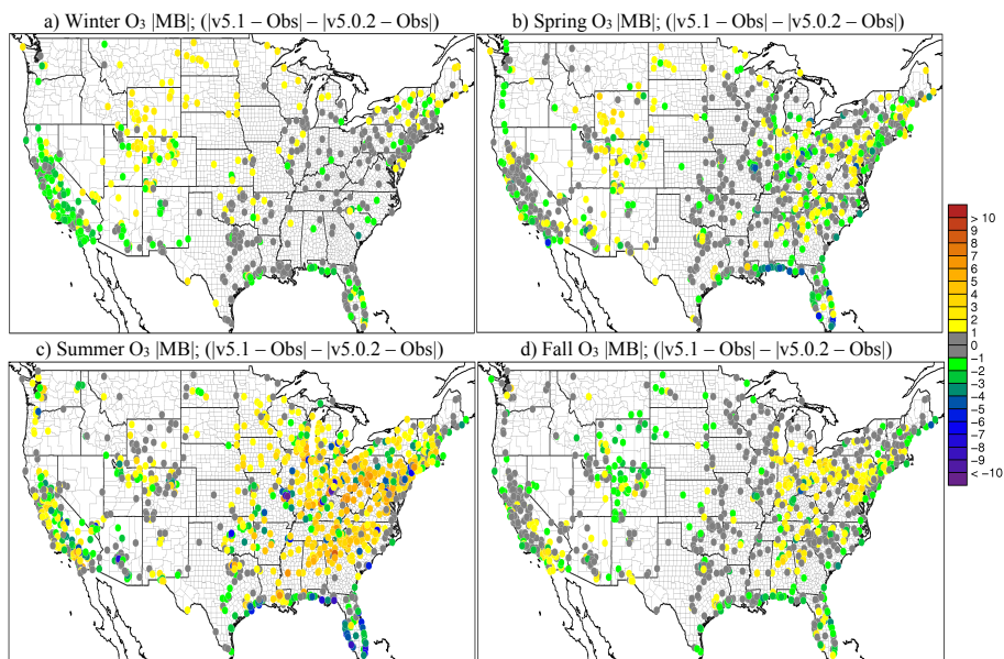
Figure 13. Difference in the absolute value of monthly average O 3 (ppbVppbv) mean bias for a) winter (DJF) b) spring (MAM) c) summer (JJA) and d) fall (SON) between CMAQ v5.0.2_Base and v5.1_Base_NEIv1 (CMAQv5.1_Base_NEIv1 - CMAQv5.0.2_Base). Cool colors indicate a reduction in O 3 mean bias in v5.1 while warm color indicate an increase in O 3 mean bias v5.1.
