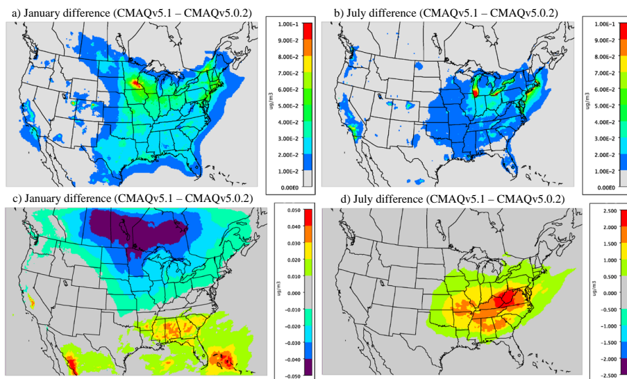
Figure 2. Monthly average sum total of AALK1, AALK2, APAH1, APAH2 and APAH3 for a) January and b) July (upper right) and the monthly average difference is the sum total of AISO1, AISO2, AISO3 and AOLGB for c) January and d) July between the aerosol treatments in CMAQ v5.0.2 and v5.1 (v5.1 - v5.0.2). All plots are in units of \mu g m^{-3} . Note that the scales for between each plot can vary.
