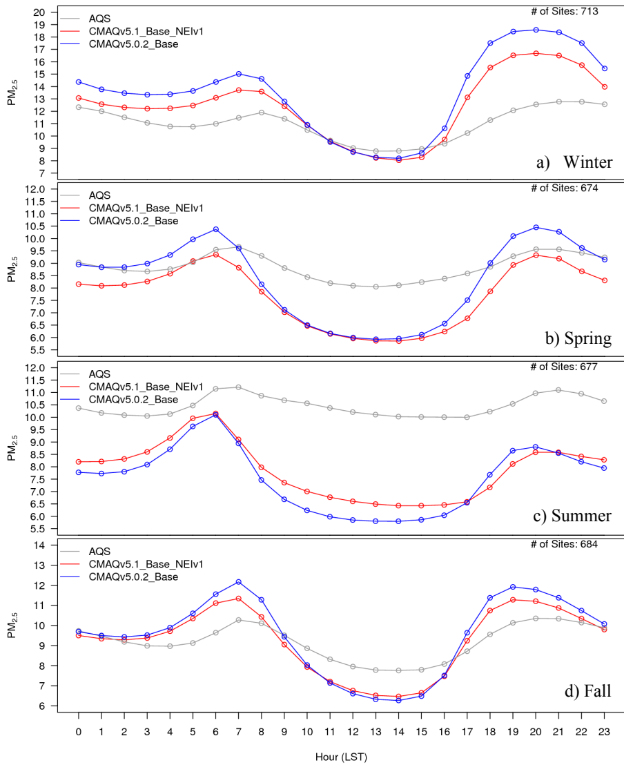
Figure 9. Diurnal time series of seasonal PM_{2.5} ( \mu g m^{-3} ) for AQS observations (grey), CMAQv5.0.2_Base simulation (blue) and CMAQv5.1_Base NEIv1 simulation (red) for a) winter b) spring c) summer and d) fall.
