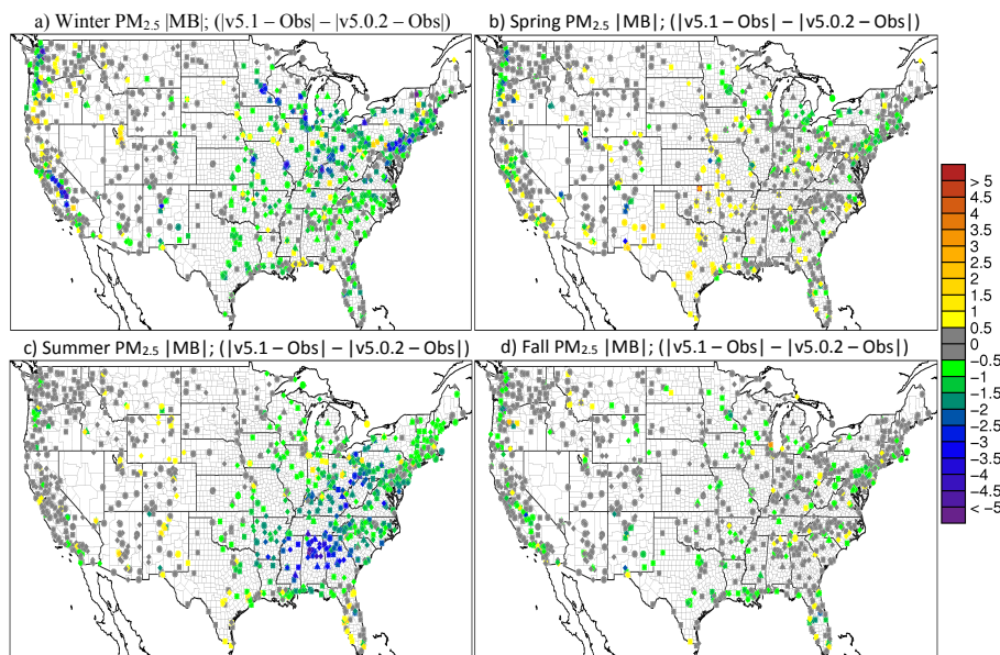
Figure 8. Difference in the absolute value of seasonal average PM_{2.5} mean bias for a) winter (DJF) b) spring (MAM) c) summer (JJA) and d) fall (SON) between CMAQ v5.0.2_Base and v5.1_Base NEIv1 (CMAQv5.1_Base NEIv1 - CMAQv5.0.2_Base). All plots are in units of \mu\text{gm}^{-3} . Cool colors indicate a reduction in PM_{2.5} mean bias in v5.1 while warm color indicate an increase in PM_{2.5} mean bias v5.1.
