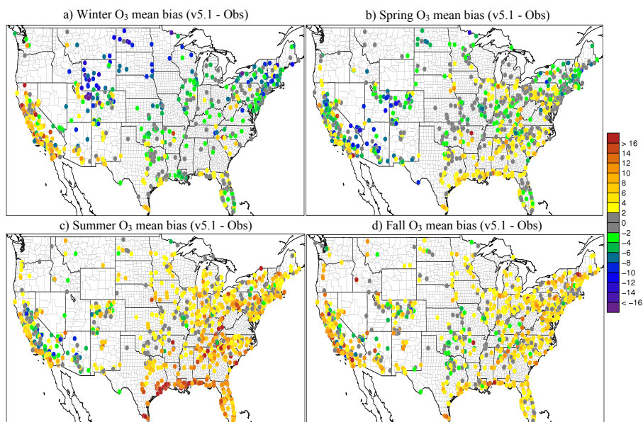
Figure 12. Seasonal average hourly O_3 ( \text{ppbVppbv} ) mean bias at AQS sites for a) winter (DJF) b) spring (MAM) c) summer (JJA) and d) fall (SON) for the CMAQ v5.1_Base_NEIv1 simulation.
