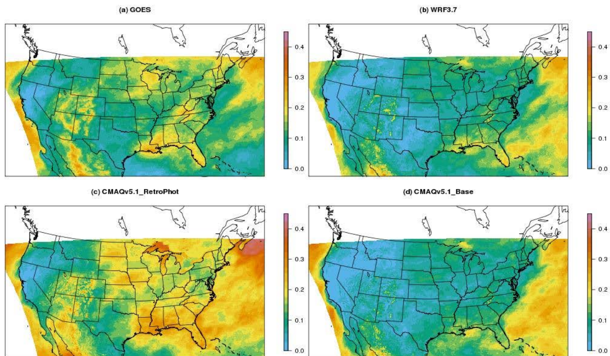
New Figure 4: The average cloud albedo during daytime hours in July 2011 with available satellite data (n = 301 hours total) derived from (a) the GOES satellite product (b) WRF3.7 (c) CMAQv5.1 with photolysis/cloud model treatment from v5.0.2 and WRF3.7 inputs (CMAQv5.1_RetroPhot) (d) CMAQv5.1 using WRF3.7 inputs (CMAQv5.1_Base).
