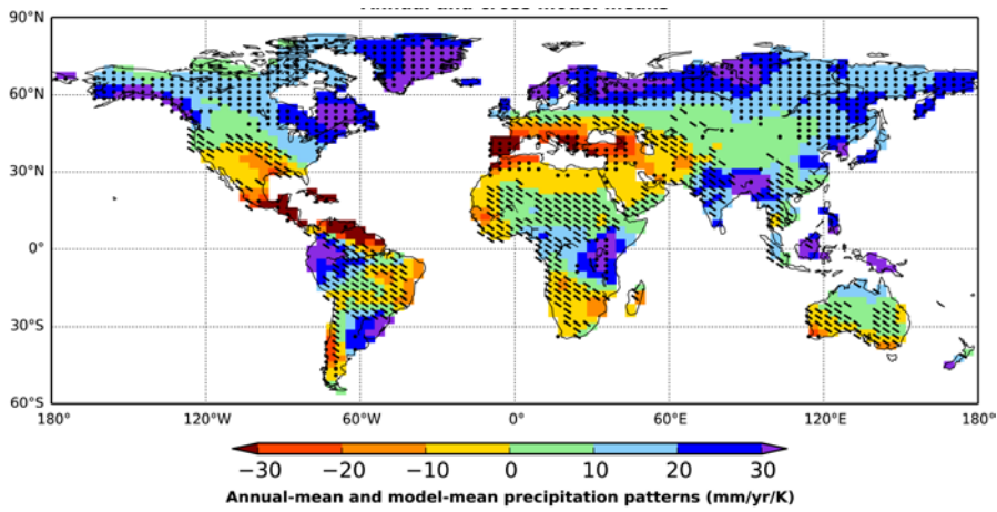
Figure S2. Annual means and variation ( 2 \times SD ) in the monthly patterns of local precipitation change per degree warming over all land ( mm\ yr^{-1}\ K^{-1} ), across 22 GCMs. In regions marked with stippling more than 66% of the models agree in the sign of the change. This figure has been prepared to enable comparison with Figure 10.9 in Meehl et al (2007).
