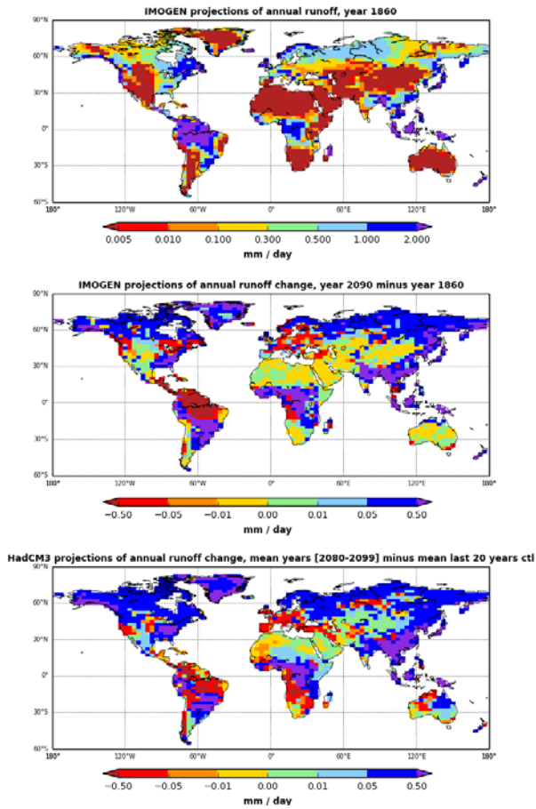
Figure 7 (Caption – figure below): Estimates of gridbox mean annual total runoff, R_{Tot} (mm/day). These are: top panel, for IMOGEN and year 1860: middle panel, IMOGEN estimates and year 2090 calculations of R_{Tot} minus those of year 1860: bottom panel, HadCM3 estimates and mean of year 2080-2099 calculations of R_{Tot} minus those of mean of last 20 years of pre-industrial control simulation.
