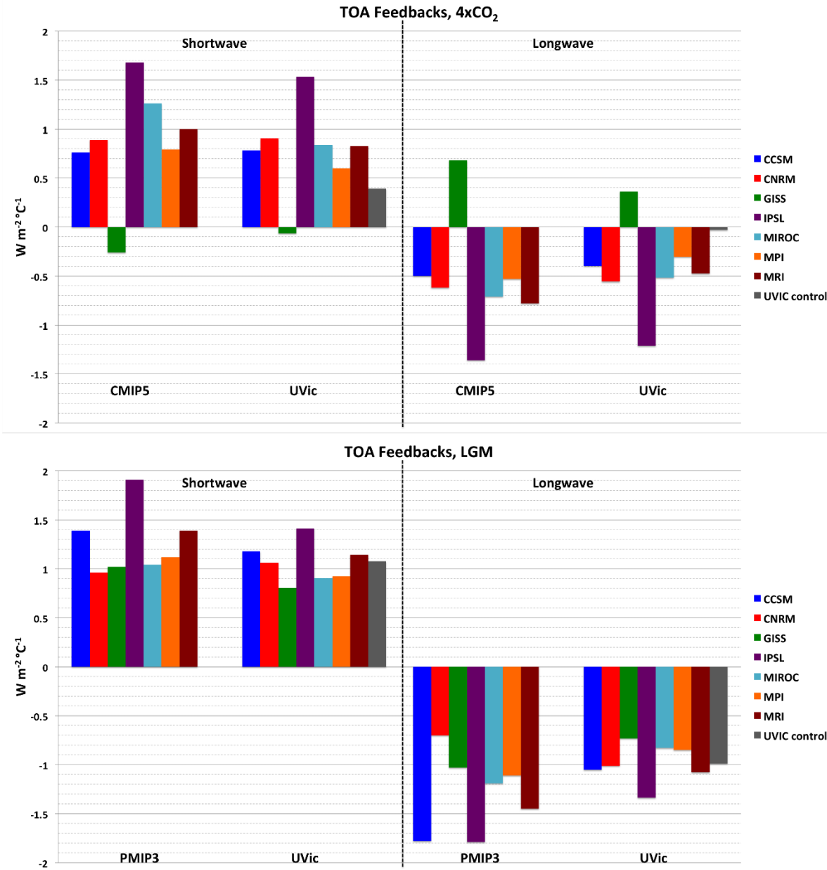
5 Figure 6: Comparison of 4xCO 2 (top) and LGM (bottom) top-of-the-atmosphere feedbacks calculated from raw CMIP5/PMIP3 output from each of the 7 GCMs (CMIP5/PMIP3) and from UVic simulations using GCMs-derived cloud feedbacks (UVic). Shortwave feedbacks are shown on the left, longwave feedbacks on the right. Positive values designate an increased forcing TO the climate system with increased temperature (i.e. positive feedback). Feedbacks from the UVic control simulation without cloud feedbacks is shown in grey.
