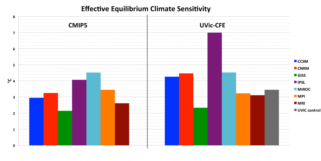
5 Figure 8: Comparison of effective equilibrium climate sensitivity ( \Delta T_{2xC,eff} ) calculated from raw CMIP5 output from each of the 7 GCMs (CMIP5) and from UVic simulations using GCMs-derived cloud feedbacks (UVic). \Delta T_{2xC,eff} from the UVic control simulation without cloud feedbacks is shown in grey.
