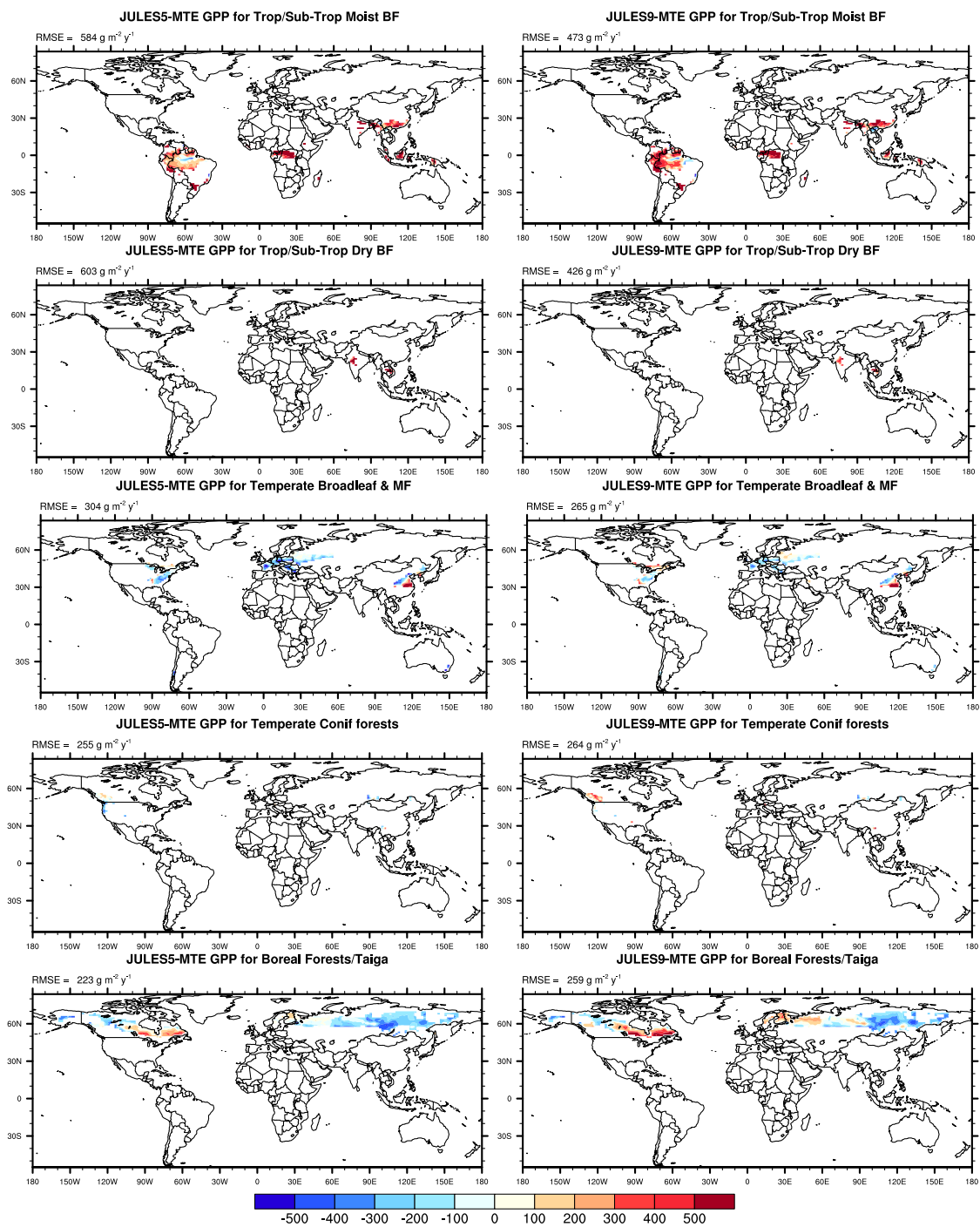
Figure S6a. Differences between JULES5 and JULES9 and the MTE GPP for each of the 11 major biomes from the WWF database (biomes with area > 1,000 km 2 ). The area-average root mean square error is given for each map.
