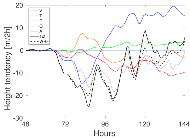
Figure 9. Time series of individual height tendency components at the 900 hPa level from the cyclone centre during the deepening period. V = vorticity advection, T = thermal advection, F = friction, Q = diabatic heating, A = imbalance term, Tot = total and WRF = WRF height tendency. Height tendencies at the cyclone centre were averaged over all grid boxes in which the 900 hPa geopotential height was less than 5 m above its minimum. In addition, the values are 2.5-hour moving averages.
