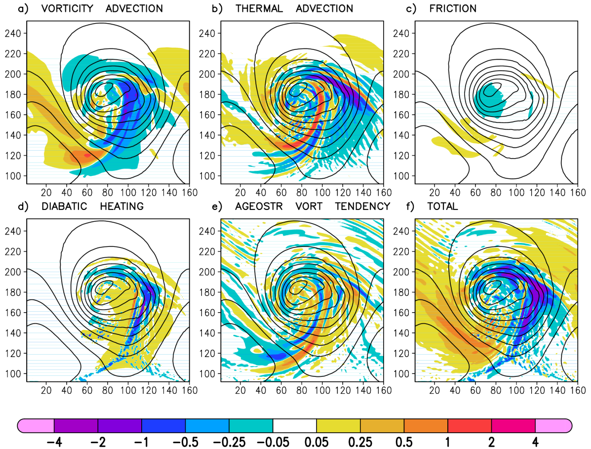
Figure 5. Vertical motions induced by individual forcing terms at level 700 hPa at time 118 h. a) \omega_V , b) \omega_T , c) \omega_F , d) \omega_Q , e) \omega_A and f) \omega_{TOT} . Unit is \text{Pa s}^{-1} and contour lines show 900 hPa geopotential height with 50 m interval.
