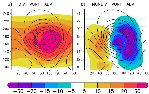
Figure 10. Height tendency associated with vorticity advection by the a) divergent and b) nondivergent winds at 900 hPa at time 118 h. Unit is \text{m} \cdot (2\text{h})^{-1} \cdot \text{m} \cdot \text{h}^{-1} .
