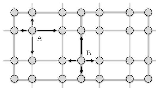
Figure 9. An illustration of how connectivity is defined in this work for nodes on a spectral element mesh. Arrows indicate connectivity for nodes A and B.
