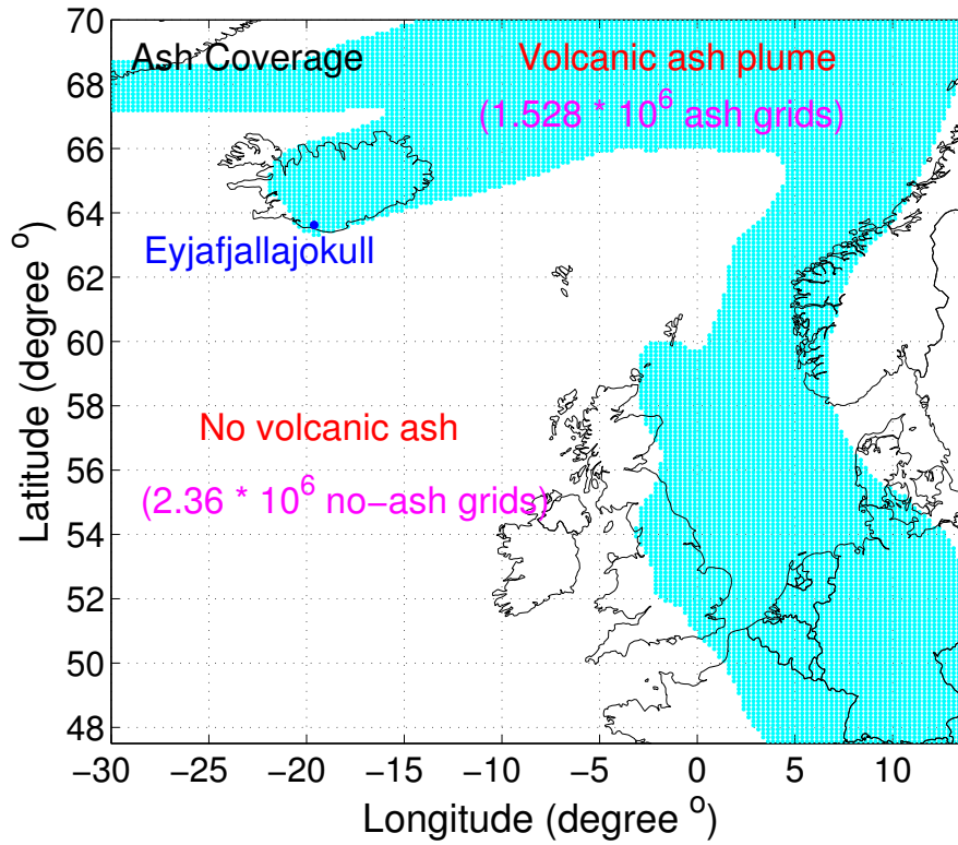
Figure 3. Characteristic of volcanic ash state.
