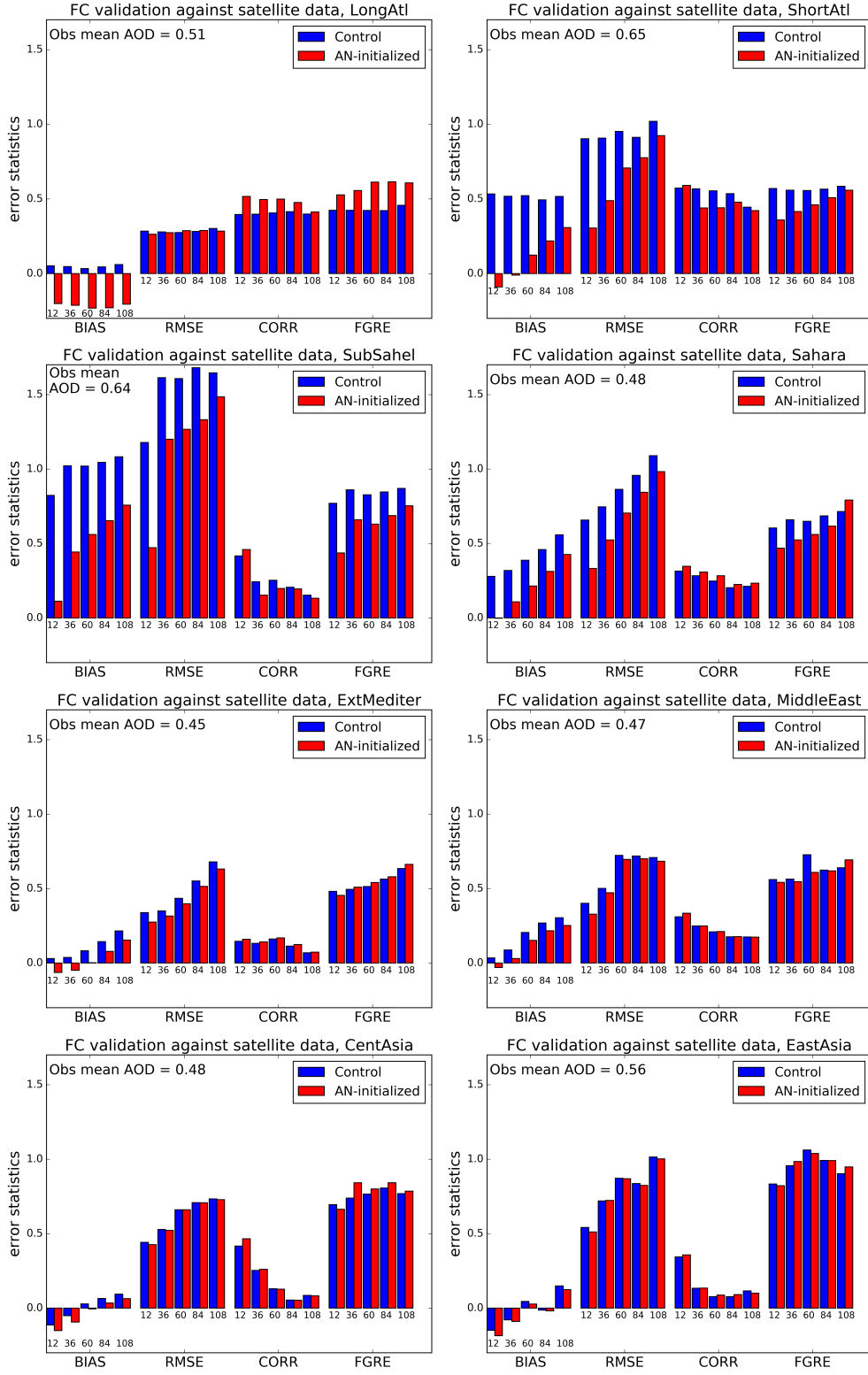
Figure 16. As the right panel of Figure 15 but for the different regional domains of Figure 5
