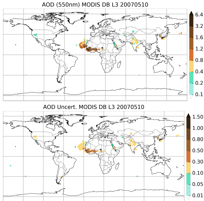
Figure 2. Aerosol optical depth (top) and its associated observation error (bottom) for May 10 2007 for the NRL MODIS Level 3 product after the application of a filter for dust-dominated conditions.
