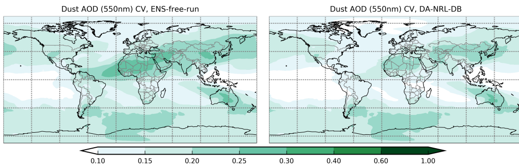
Figure 8. Coefficient of variation for the month of May 2007 for the ENS-free-run (left) and DA-NRL-DB (right) experiment, when the ensemble is created perturbing the emitted mass vertical flux for each dust bin.
