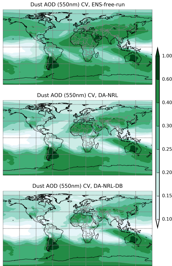
Figure 7. Coefficient of variation for the month of May 2007 for the ENS-free-run (top), DA-NRL (centre) and DA-NRL-DB (bottom) experiment, when the ensemble is created perturbing the emitted mass vertical flux for each dust bin and the threshold on the friction velocity generating dust horizontal flux.
