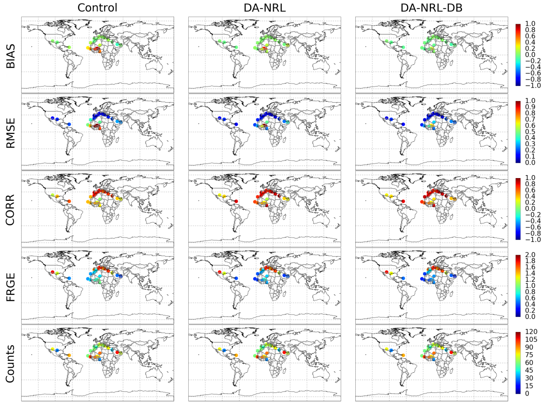
Figure 12. Maps of validation statistics: BIAS, RMSE, CORR, FRGE for the Control (left), DA-NRL (centre) and DA-NRL-DB (right) experiment calculated against AERONET AOD for a selection of stations providing observations during the study period (May to August 2007). Maps of the observation counts used for validation are shown in the bottom row.
