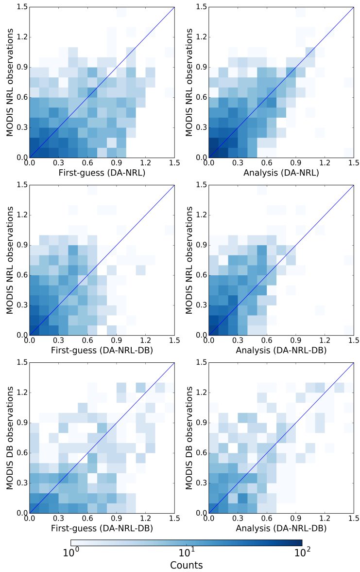
Figure 9. Binned scatter plots of the counts of the logarithm of assimilated observations and first-guess (left plot) and analysis (right plot) for the DA-NRL experiment (top row) and DA-NRL-DB experiment (central and bottom rows), calculated for May to August 2007. A logarithmic scale is used for the counts.
