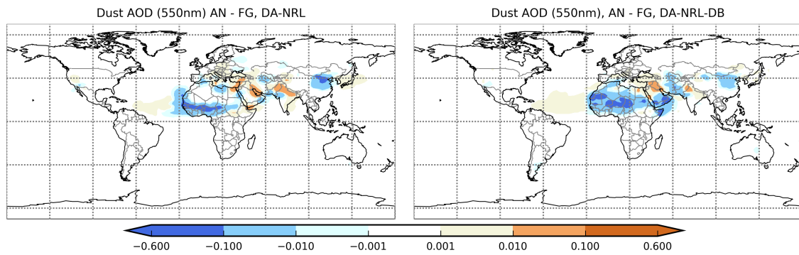
Figure 10. Mean dust AOD analysis increments for May to August 2007 at 12 UTC for the DA-NRL experiment (left) and for the DA-NRL-DB experiment (right).
