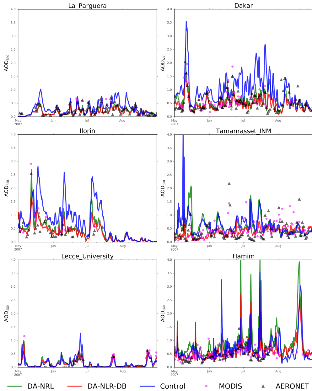
Figure 11. Time-series of AOD values for May and August 2007 in La Parguera (top left), Dakar (top right), Ilorin (centre left), Tamanrasset INM (centre right), Lecce University (bottom left), and Hamim (bottom right) for Control (blue), DA-NRL (green), DA-NRL-DB (red) experiment, for MODIS AOD (NRL and DB; magenta circles), and for AERONET AOD (black triangles) in dust-dominated conditions. Analysis values are used for the data assimilation experiments.
