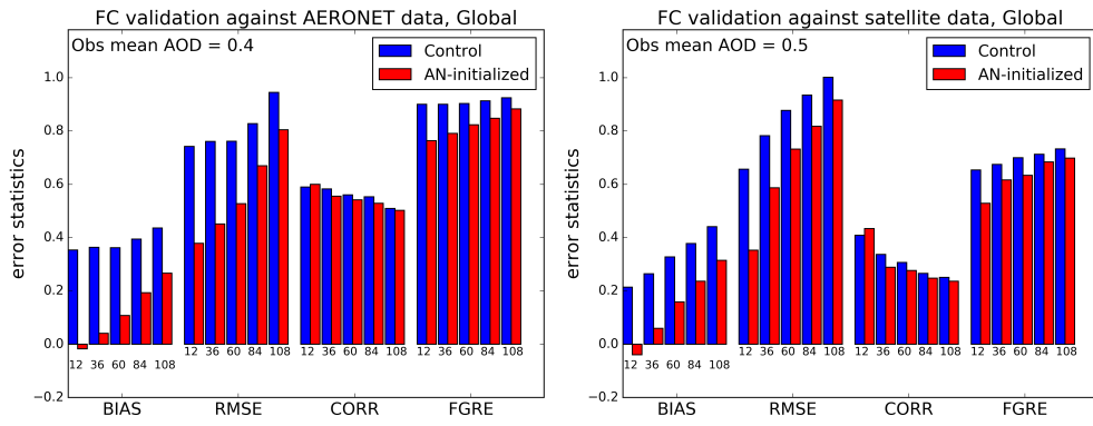
Figure 15. BIAS, RMSE, CORR, and FGRE for the forecast at 12, 36, 60, 84 and 108 hours of the Control (blue) and AN-initialized (red) experiment, i.e. the experiment initialized with the DA-NRL-DB analysis, calculated against AERONET observations (left) and against global satellite retrievals, both NRL MODIS and MODIS Deep Blues, (right) filtered for dust-dominated conditions. The AERONET stations are the ones in Figure 5. The dust mean AOD for the observations used to validate the 12 hour forecast during the experiment period is also reported.
