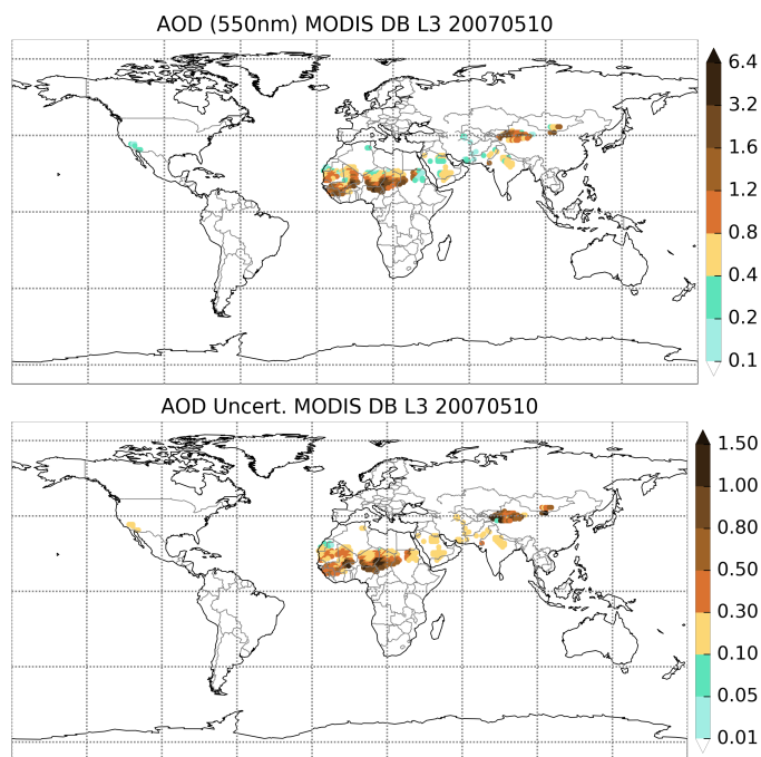
Figure 3. Aerosol optical depth (top) and its associated observation error (bottom) for May 10 2007 for the MODIS Deep Blue Collection 6 Level 3 product after the application of a filter for dust-dominated conditions.
