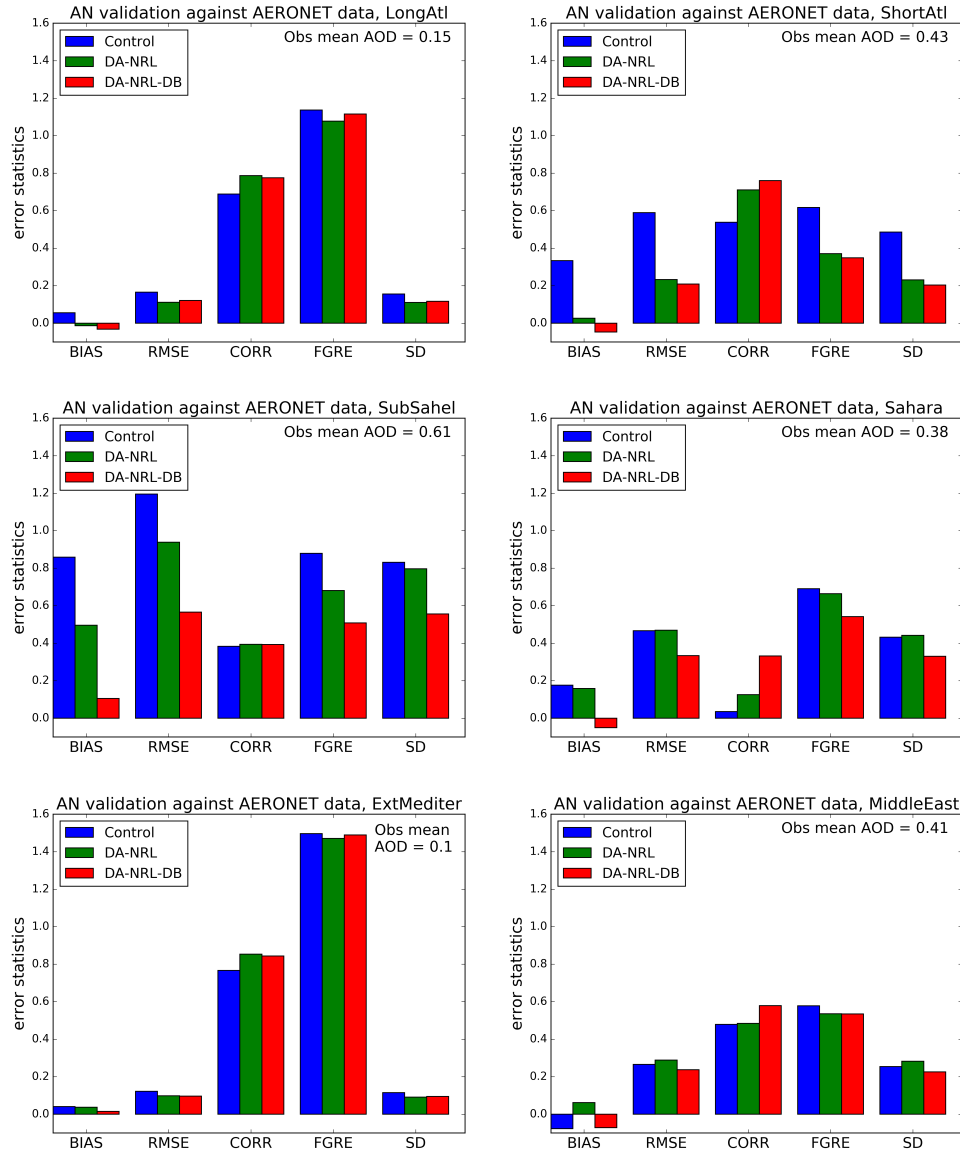
Figure 14. BIAS, RMSE, CORR, FRGE and SD for the Control experiment, the DA-NRL experiments and the DA-NRL-DB experiment calculated against AERONET observations for groups of stations within the regional domains in Figure 5. The dust mean AOD for the observations used for validation during the experiment period is also reported.
