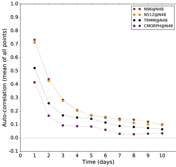
c. IO domain (60°–80°E, 10°S–10°N)
