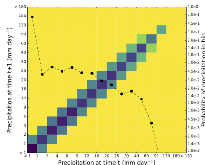
f. N1024e@N48 WP region
