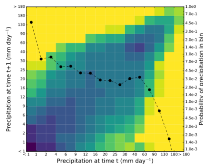
c. CMORPH@N48 NWP region
