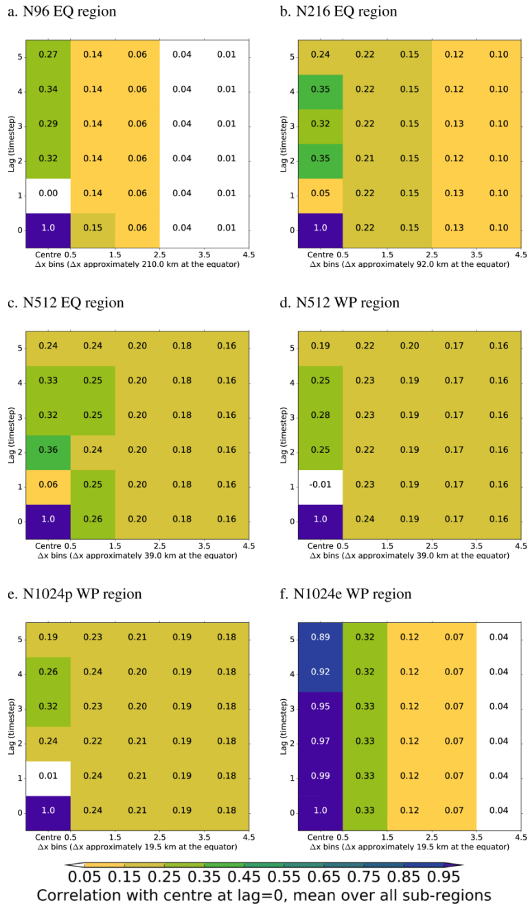
Figure 3. For each model and using time-step precipitation on the native horizontal grid, filled boxes and numbers show the lagged correlations between the central grid-box in each 7x7 sub-region and grid-boxes within each range of distance on the horizontal axis (in units of the longitudinal grid spacing at the equator, \Delta x ) away from the central point, averaged over all 7x7 regions.
