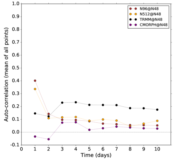
d. SC domain (103°–119°E, 23°–32°N)
