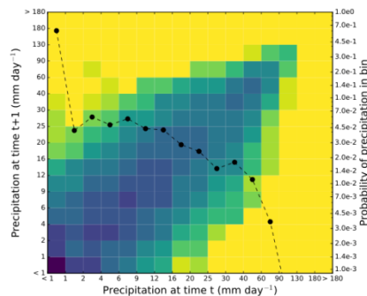
i. N1024e@N48 WP region
