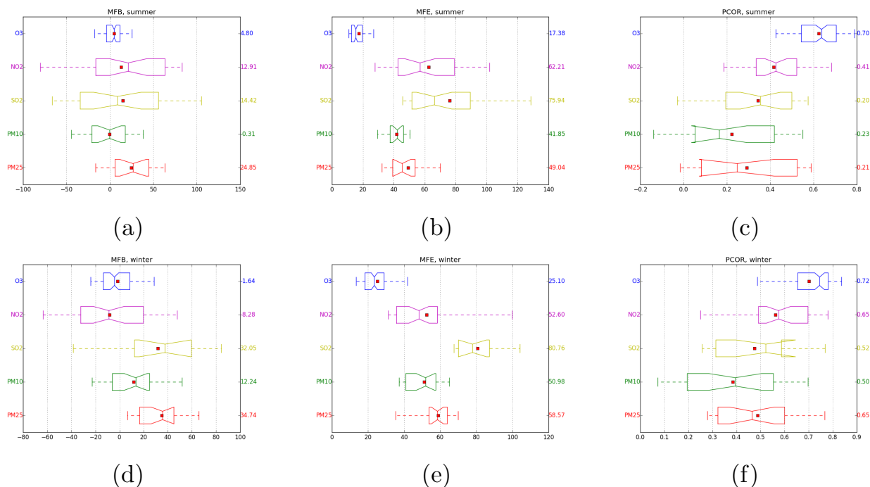
Figure 8. Performance statistics for the main model species and for daily averaged values. The numbers on the right axes give the overall scores (Pearson’s correlation, MFE, and MFB), while the box plots show the variability among the EMEP stations. The boxes extend from the lower to upper quartile values of the data. The center lines show the medians, and the red squares show the means over stations. The whiskers indicate the 5 and 95 percentile values, and the values on the right axis of each panel are the overall value of the considered indicator, i.e. merging all the stations into a single statistical dataset as described in Jacobson (2005)
