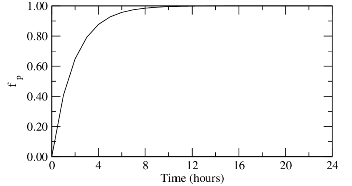
Figure 7. Function defined to moderate the mineral dust emissions fluxes after a precipitation event.
