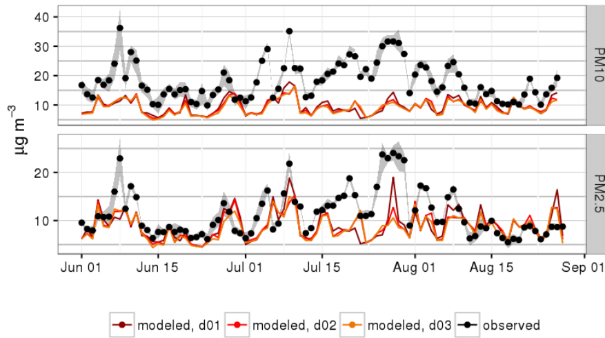
Figure 12. Daily mean PM_{10} and PM_{2.5} concentrations as observed and modeled (base run) at urban background stations in Berlin. Daily means are averaged over five stations for PM_{10} and four stations for PM_{2.5} . The grey shaded areas represent the variability between the different stations, showing 25th and 75th percentiles. Model results are given for all three model domains (d01 - 15km horizontal resolution, d02 - 3km, d03 - 1km).
