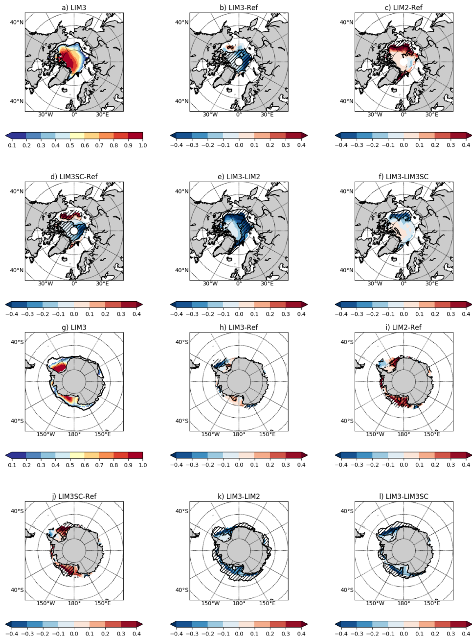
Figure 1. Geographical distribution of Arctic sea-ice concentration averaged for September (a–f) and Antarctic sea-ice concentration averaged for March 2003–2012 (g–l). (a, g) show values simulated by LIM3, while (b, h) show LIM3 difference with Meier et al. (2013) passive microwave observations, (c, i) the corresponding LIM2 difference, (d, j) the LIM3SC difference, while (e, k) show the difference between LIM3 and LIM2 and (f, l) the difference between LIM3 and LIM3SC. Sea-ice concentration differences are computed only where both values are present. Only areas where the sea-ice concentration is greater than 15% are plotted. In (a, e), thick black lines show the observed Meier et al. (2013) sea-ice edge as the 15% sea-ice concentration isopleth. Hatching indicates regions with statistically significant differences at the 5% level, based on unequal variances t-test.
