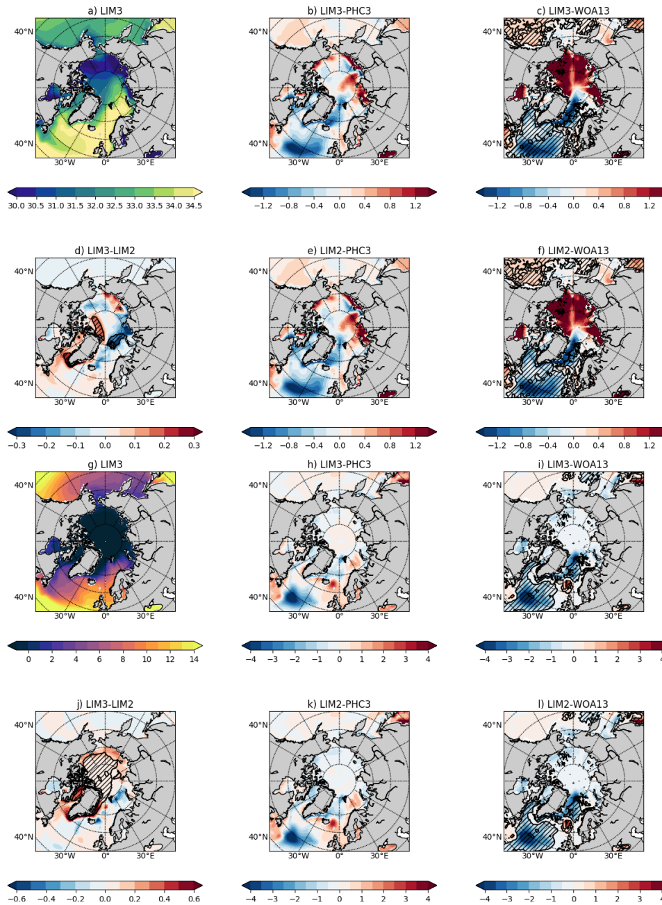
Figure 5. (a–f) Arctic sea-surface salinity in psu (SSS) and (g–j) sea-surface temperature in ^{\circ}\text{C} (SST) averaged over the period of 2003–2012. (a, g) show the LIM3 averages, (b, h) the difference between PHC3 (Steele et al., 2001) and LIM3, (c, i) the difference between WOA13 (Boyer et al., 2013) and LIM3, (e, f, k, l) the corresponding differences for LIM2, and (d, j) show the differences between LIM3 and LIM2. WOA13 data are averaged over the years 2005–2013, while PHC3 data contain observations from 1900–1998, as in WOA98, plus all Arctic observations until 2004. Hatching indicates regions with statistically significant differences at the 5% level based on unequal variances t-test. As PHC3 does not include standard deviation and sample size, the statistical significance levels of LIM–PHC3 differences could not be estimated.
