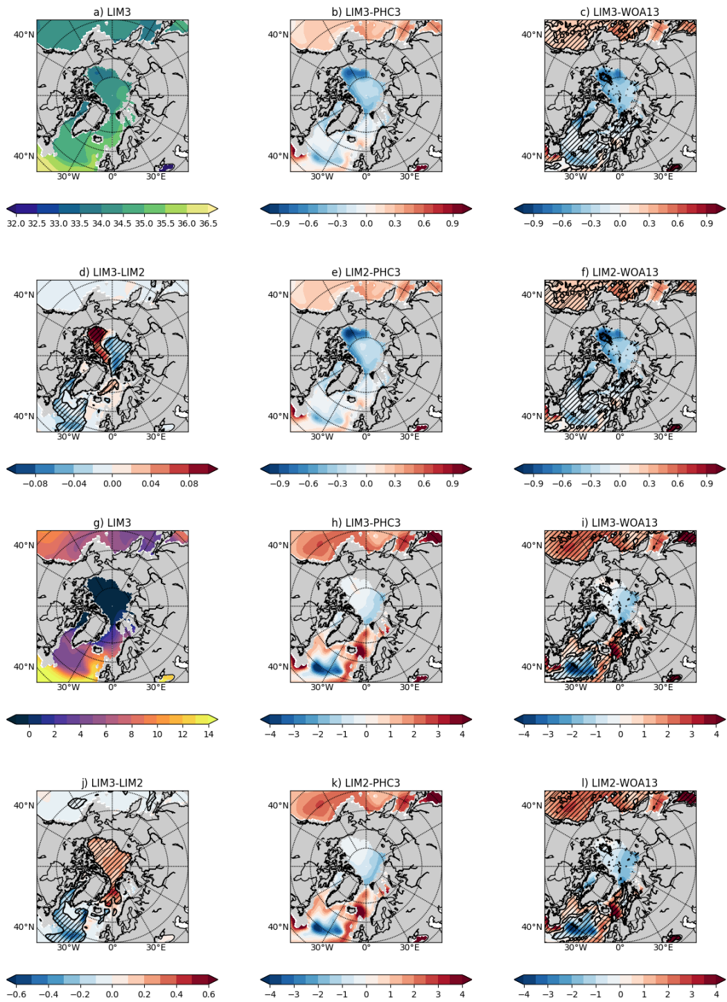
Figure 7. As Figure 5, but for the Arctic intermediate water (AIW) at 250 m.
