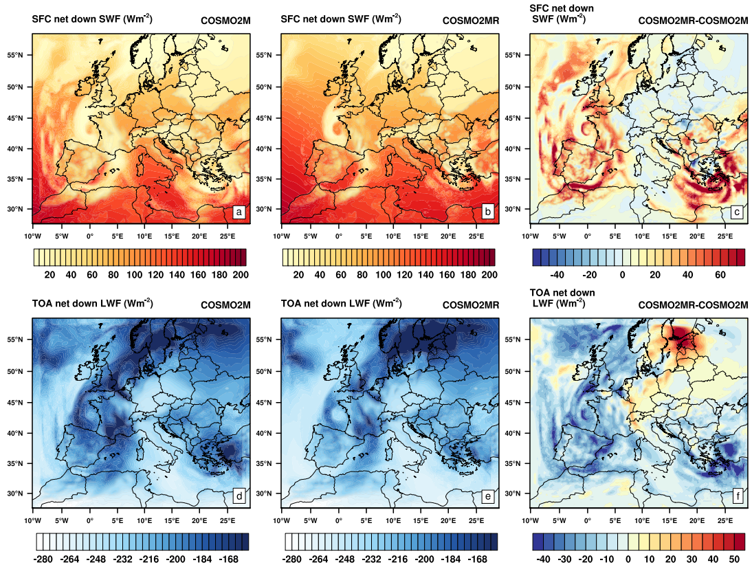
Figure 7. Comparison and difference between short wave and long wave radiation fluxes surface and top of the atmosphere, and it is difference between two simulation (COSMO2MR radiation coupled minus COSMO2M).
