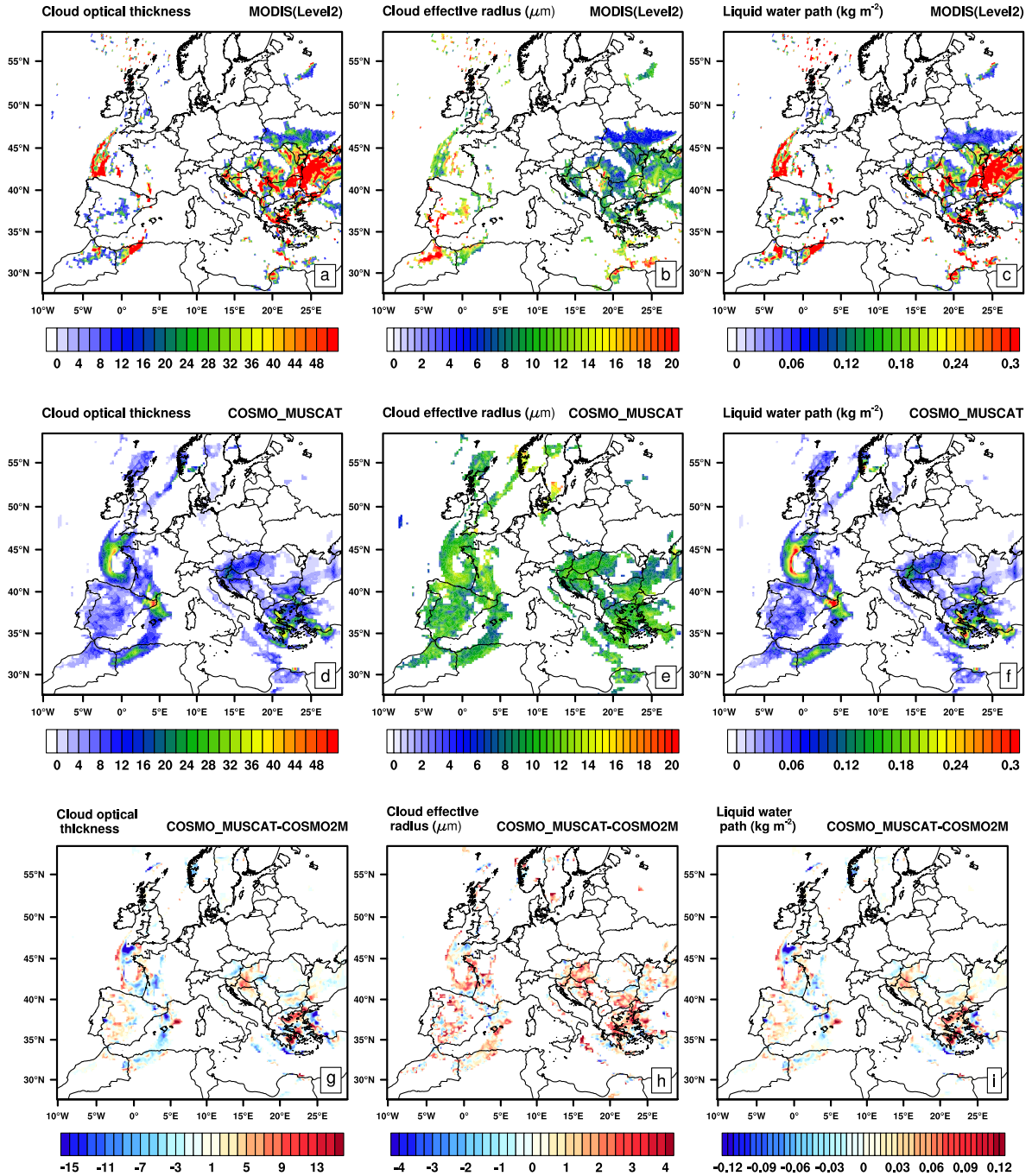
Figure 4. MODIS Level-2 (a) cloud optical depth, (b) cloud effective radius, (c) cloud water path, COSMO-MUSCAT derived (averaged between 8.00 - 14.00 UTC, approximate MODIS-Terra overpass time over the domain) (d) cloud optical depth, (e) cloud effective radius, (f) cloud water path, and difference between COSMO-MUSCAT and COSMO2M simulations (g,h,i), for 17 February 2007.
