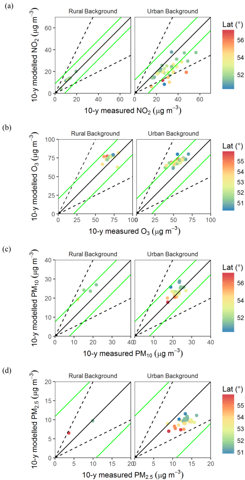
Figure 1: Scatter plots of the 10-year means of the modelled and measured pollutant daily metrics at each site, grouped by site type, and with data markers shaded according to the latitude of the measurement site: (a) NO 2 ; (b) O 3 ; (c) PM 10 ; (d) PM 2.5 . The values of r , FAC2, NMB and RMSE associated with the data in each plot are given in Table 1. The solid and dashed lines are the 1:1, and the 2:1 and 1:2 lines, respectively. The green lines bound the respective model quality objective calculated using the formulae published in FAIRMODE project WG 1 documents at http://fairmode.jrc.ec.europa.eu (as at March 2017) and allowing for variable measurement uncertainty using the measured values in this study. See main text for further details.
