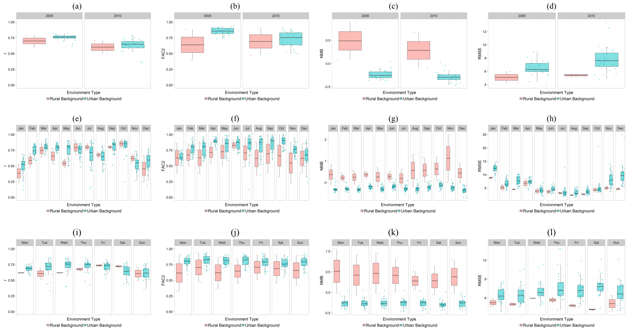
Figure 5: Model-measurement statistics per site for PM_{2.5} daily mean concentrations during 2009-2010, by site type, and by (a-d) year, (e-h) month of year, and (i-l) day of week. (a), (e) and (i) are Pearson's correlation coefficient ( r ); (b), (f) and (j) are fraction of data pairs within a factor of two (FAC2); (c), (g) and (k) are normalised mean bias (NMB); and (d), (h) and (l) are root mean squared error (RMSE) in \mu g m^{-3} . Dots show individual site statistics ( n = 2 and 28 for RB and UB sites respectively), which are summarised in the superimposed box-plot whose shading demarcates the interquartile range (IQR) and whose whiskers extend to the largest and smallest value within 1.58 \times IQR from the box hinges.
