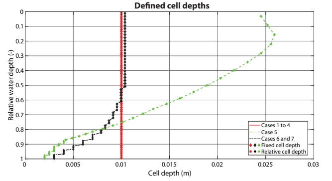
Figure 4. Defined cell depths for the Cases 1 to 7. For plotting reasons, the vertical axis displays the depth from the water surface relative to the local water depth. The cell depths that are defined relative to the local water depth (as marked by *) are displayed for the average water depth in each case study.
