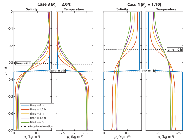
Figure 5. Interface positioning over time, displayed on the depth profiles of S and T (both in \text{kgm}^{-3} relative to the reference density), for the density ratios R_{\rho} = 2.04 (Case 3) and R_{\rho} = 1.19 (Case 4). The depth profiles are averaged over the complete horizontal domain and represent the simulations without a turbulence model.
