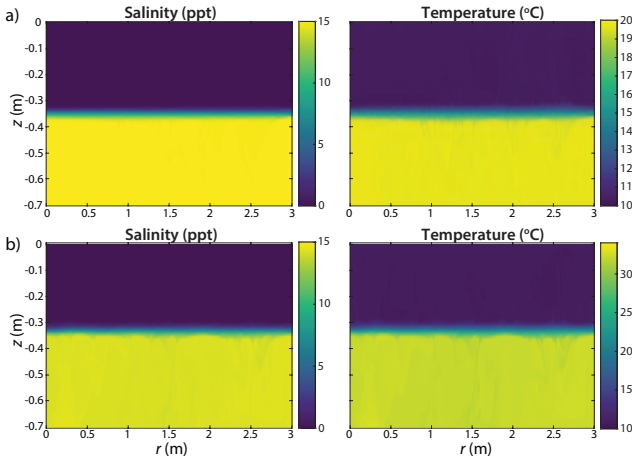
Figure 7. Double-diffusive convection in a layered system with a cold and fresh layer on top of a warm and saline water ( t = 4500 s since the start), with density ratios of a) R_\rho = 0.15 (Case 1), and b) R_\rho = 0.50 (Case 2). All figures represent simulations without the use of a turbulence model.
