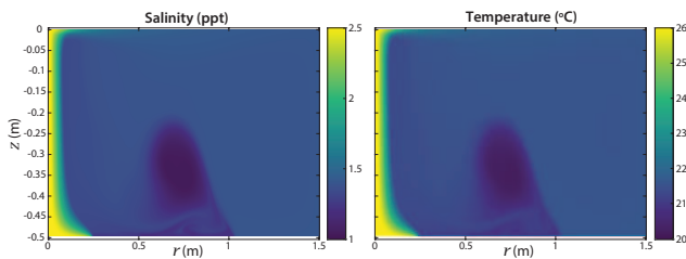
Figure 16. Unstable system (Case 7) with denser cold and fresh water on top of a warm and saline inflow ( t = 5400 s since the start). The inflowing water flows upward through the centre, independent of the inflow velocity.
