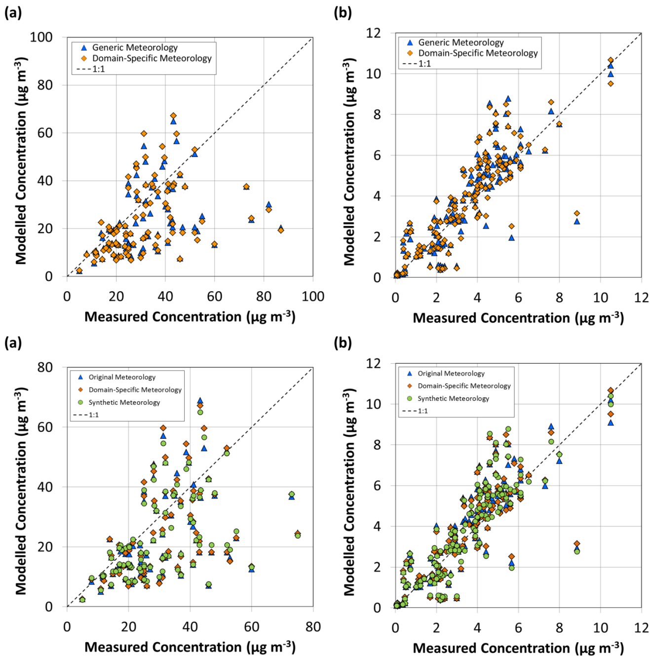
Figure 5: Modelled concentrations plotted against measured values for all sites for (a) NO 2 and (b) NH 3 using both the generic meteorological dataset (LYNE95) and original meteorology (as in Figure 4) and using the domain-specific and synthetic meteorological data. Plot data provided in the supplementary material datasets.
