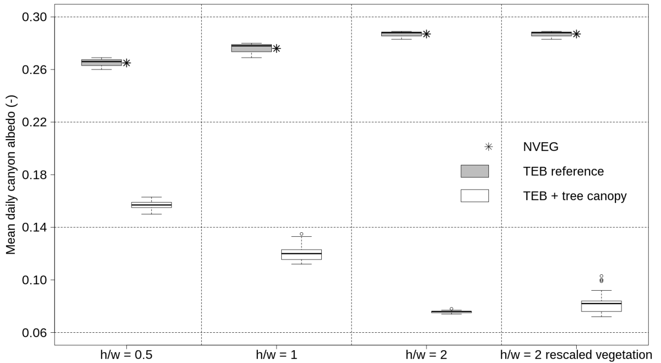
Figure 9. Comparison of the mean daily canyon albedo between the reference TEB simulations without distinction between low and high vegetation and the new version including a tree canopy by aspect ratios for all seasons, orientations and vegetation layouts confounded. See section 5.2.1 and Fig. 2 for further explanations about the h/w = 2 rescaled vegetation configurations.
