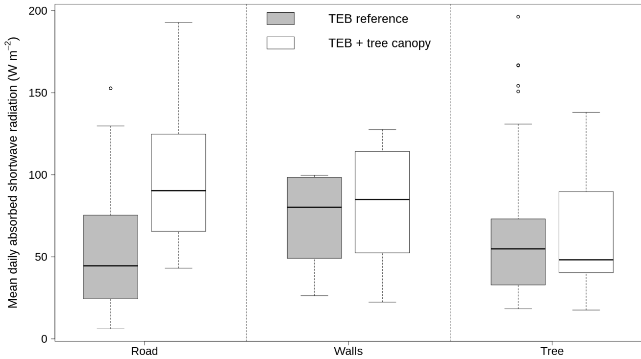
Figure 8. Comparison of mean daily total shortwave radiation flux ( W m^{-2} ) absorbed by road, walls, and tree between the reference TEB simulations without distinction between low and high vegetation and the new version including a tree canopy by surface for all seasons, aspect ratios, orientations and vegetation layouts confounded.
