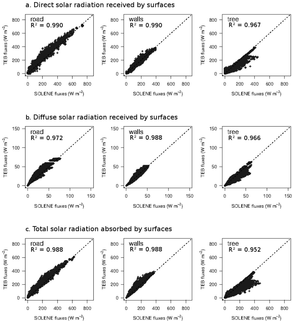
Figure 7. Scatterplots comparing TEB and SOLENE simulations of hourly direct (top) and diffuse (middle) solar radiation fluxes ( W m^{-2} ) received by facets before multiple reflections and total shortwave radiation fluxes ( W m^{-2} ) absorbed by facets after interreflections (bottom), for urban canyons with vegetation. Each scatterplot gathers the hourly fluxes simulated for the four seasons, the four aspect ratios, and the four street orientations.
