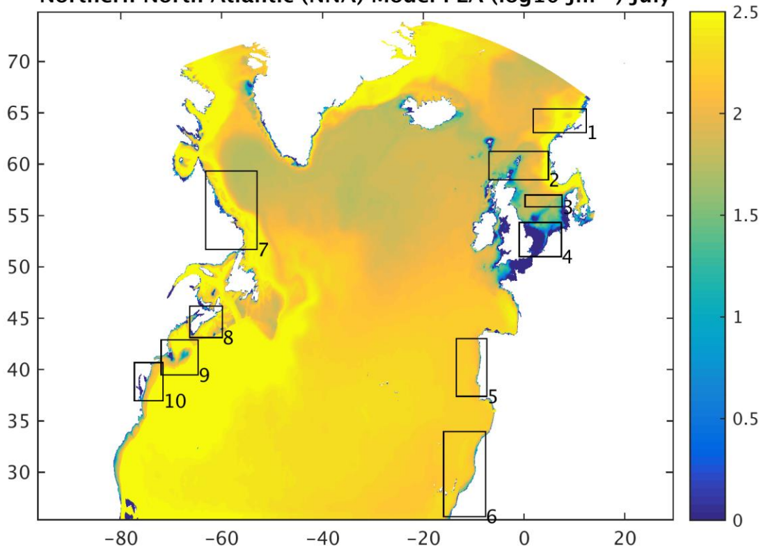
Northern North Atlantic (NNA) Model PEA ( \log_{10} \text{Jm}^{-3} ) July
