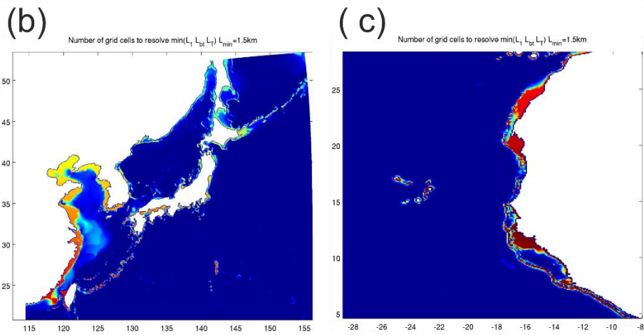
5 Figure 7 An example of how a 1/12^\circ global grid (a) might conceptually be refined to resolve the dominant scales. Parameter shown is number of cells needed in each global grid cell to resolve these scales down to a minimum scale of 1.5km, so ranges from 1 (no refinement) to (72/12)^2=36 . Below are two example in more detail for (b) East Asia and (c) NW Africa.
