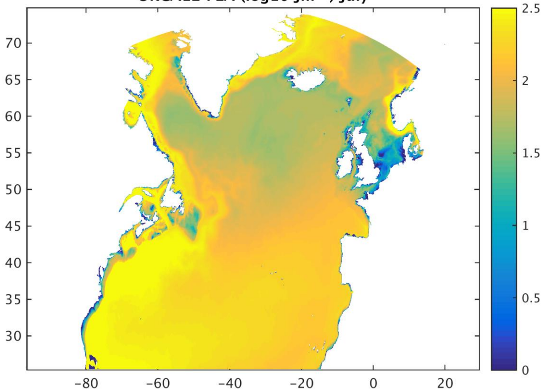
5 Figure 5 Potential energy anomaly (PEA; Eqn 2) for July (mean 1985-2003; note log scale) for the Northern North Atlantic (NNA) NEMO configuration (TOP; including tides and k- \epsilon (GLS) mixing) and global ORCA12 model (BOTTOM; with the TKE mixing scheme and no tides). Also shown are regions 1-10 used for a seasonal analysis (Figure 6).
