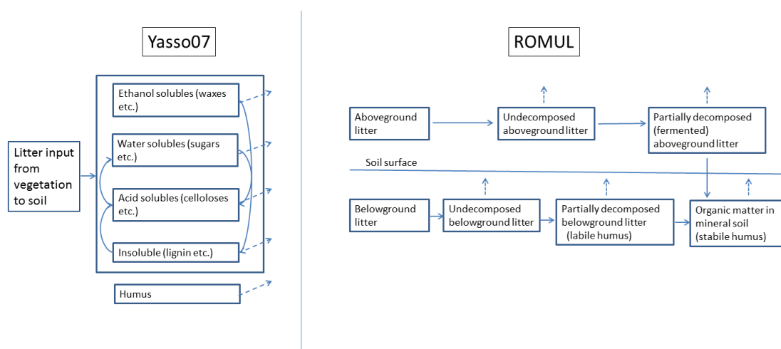
Figure 1: Schematic illustration of Yasso07 (left) and ROMUL (right) soil carbon models. Solid arrows indicate fluxes of organic matter, while dashed arrows indicate CO 2 fluxes to atmosphere.
