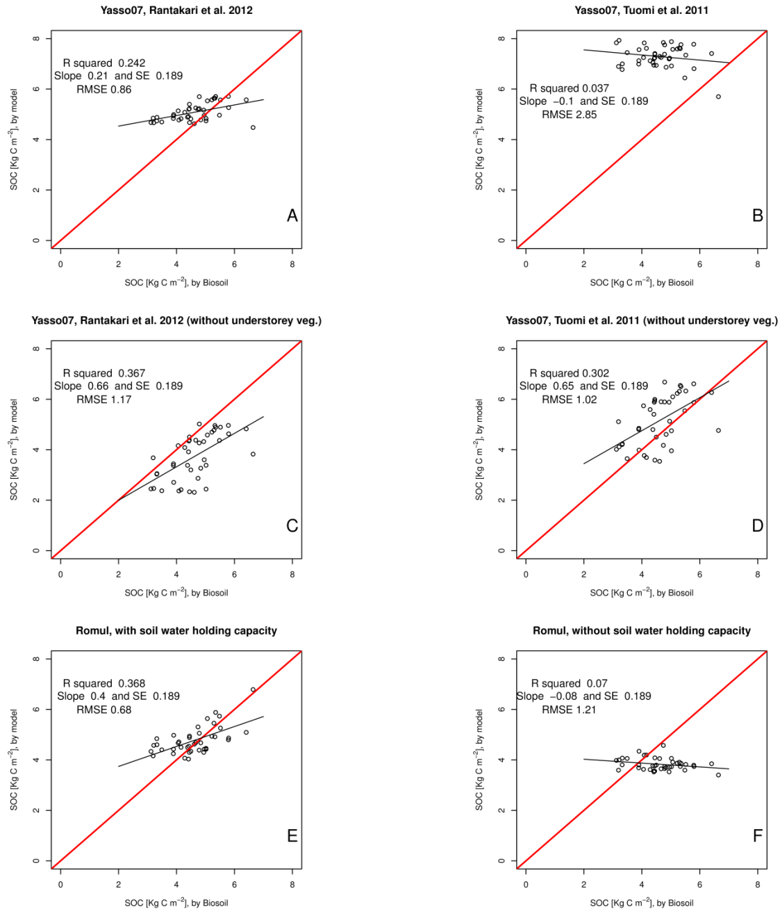
5 Figure 6. One-by-one plots for mean model estimates and mean Biosoil measurements of soil carbon stocks for 41 latitudinal bands across Finland. Panel A is Yasso07 with Rantakari et al. (2012) parameters, while B is with Tuomi et al. (2011) parameters. C and D are same as A and B but without understorey litter input. E and F are with ROMUL model where E is with soil water holding
