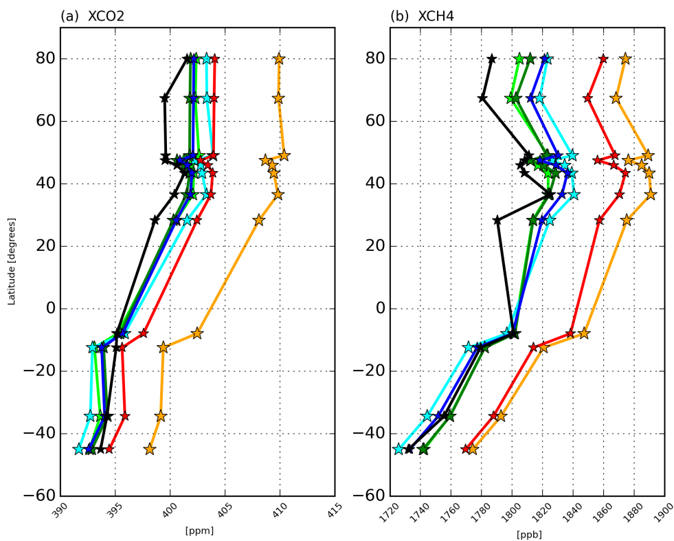
Figure 8. Comparisons of latitudinal distribution of (a) XCO 2 and (b) XCH 4 as derived from monthly mean (7 March to 10 April) TCCON sites (black, see Table 2)) and simulations using different mass fixers at different resolutions: red/orange without mass fixer at low/high resolutions blue/cyan with the proportional mass fixer at low/high resolutions; and green/light green with the Bermejo & Conde fixer and low/high resolutions respectively. See Table 1 for a more detailed description of the experiments.
