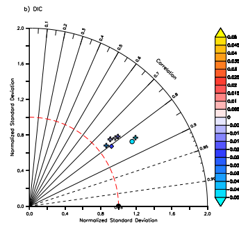
Figure 13. Taylor diagram assessing the alkalinity (a) and DIC (b) of the ACCESS-ESM1 simulation (circle), the median of CMIP5 models (diamond), and the individual members of the CMIP5 ensemble (crosses) with observations.
