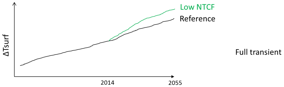
Figure 1: Schematic of future coupled-ocean simulations based on the SSP3-7.0 scenario.
