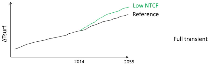
Figure 1: Schematic of future coupled-ocean simulations based on the SSP3-7.0 scenario.
