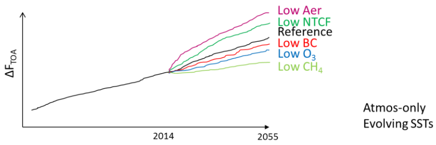
10 Figure 2: Schematic of future prescribed SST simulations based on the SSP3-7.0 scenario.
