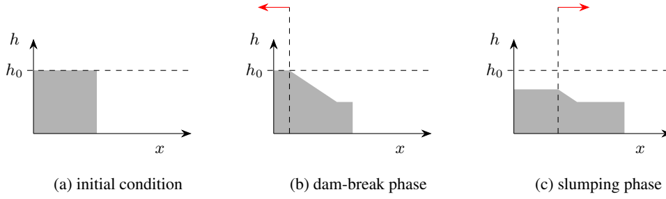
Figure 2. Schematic diagram of the lock-release static initial condition (a) and the following dam-break (b) and slumping (c) phases with shock wave propagation direction indicated ( \rightarrow ).
