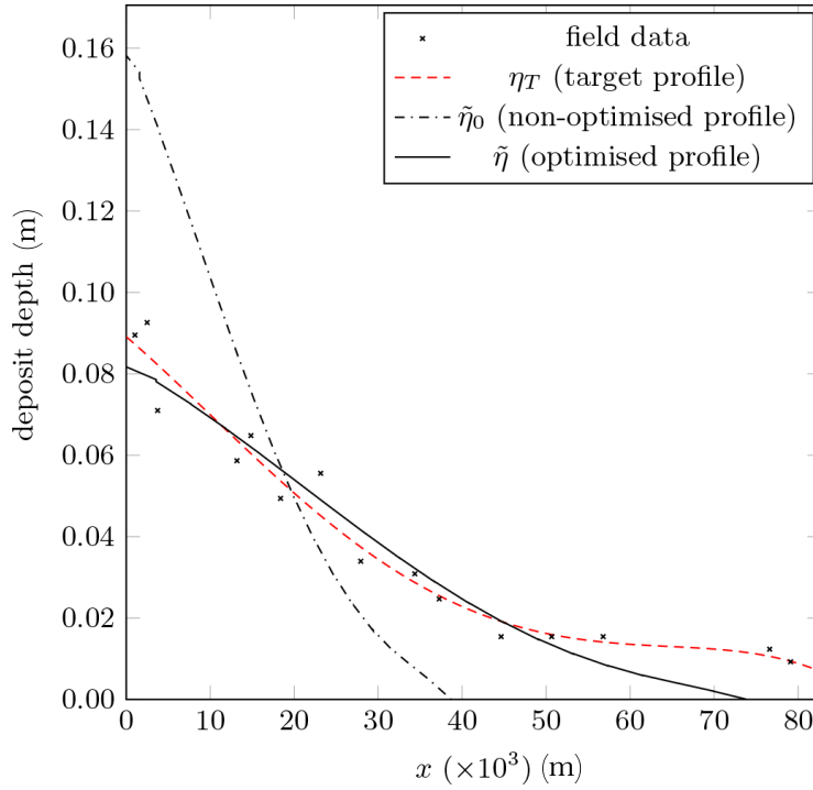
Figure 7. Dimensional deposit output \tilde{\eta}_0 from initial parameter guess (73), and optimised dimensional deposit output \tilde{\eta} from the optimised parameter (76), shown against the field measurement from Bed 1.1 (Talling et al., 2007a) and fourth-order polynomial target deposit profile, \eta_T .
