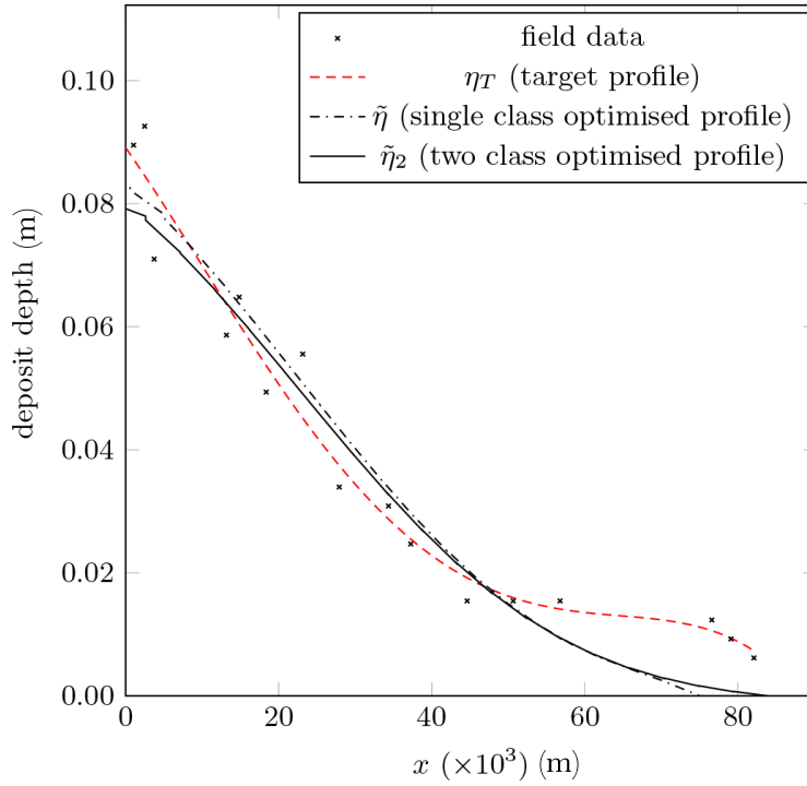
Figure 10. Optimised dimensional deposit output from the model with both mud and sand sediment classes, \tilde{\eta}_2 shown against the optimised results from the single sediment class model, \tilde{\eta} , the field measurement from Bed 1.1 (Talling et al., 2007a) and fourth-order polynomial target deposit profile, \eta_T .
