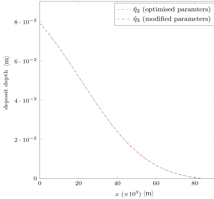
Figure 11. Optimised dimensional deposit output from the model with both mud and sand sediment classes, \tilde{\eta}_2 shown against results from the same model, with the same parameters but a mud settling velocity reduced by two orders of magnitude, \tilde{\eta}_3 .
