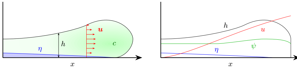
Figure 1. Schematic representation of a dense gravity current (left), and a corresponding depth-averaged shallow water approximation (right), shows current height h , volume fraction c , and depth-averaged volume fraction \psi , velocity u , and forward component of the depth-averaged velocity u , and deposit depth \eta .
