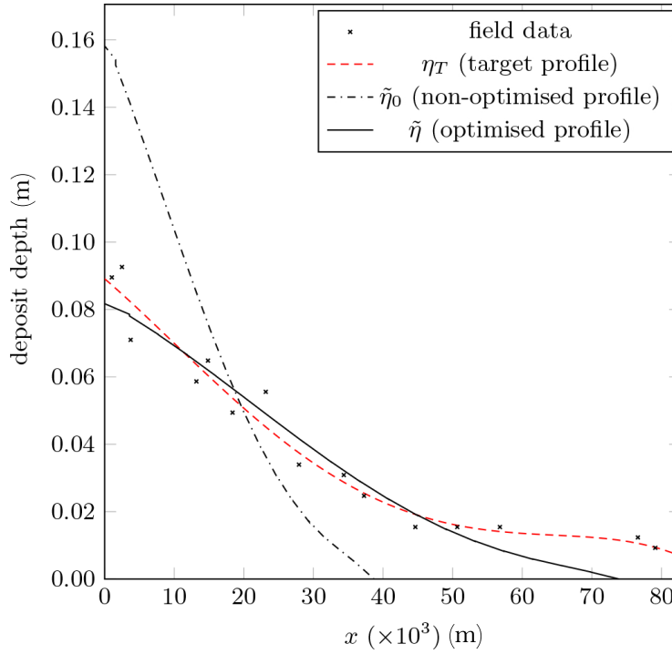
Figure 7. Dimensional deposit output \tilde{\eta}_0 from initial parameter guess \tilde{\eta}_0 (73), and optimised dimensional deposit output \tilde{\eta} from the optimised parameter (76), shown against the field measurement from Bed 1.1 (Talling et al., 2007a) and fourth-order polynomial target deposit profile, \eta^T .
