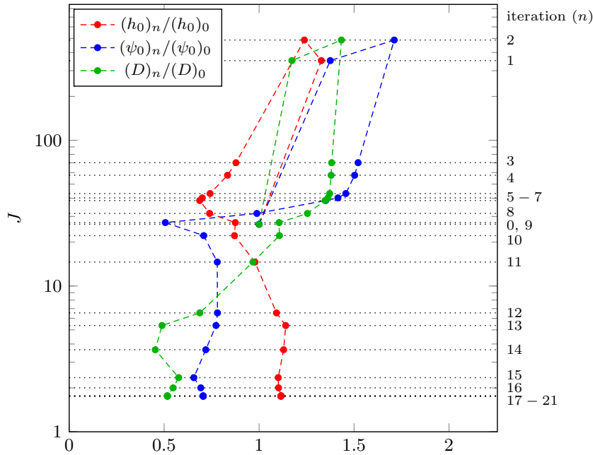
Figure 6. Values of parameters over the optimisation iterations against the value of the objective functional, J , that we are aiming to minimise. Values shown are normalised by their starting values. (*)_n is the value of parameter * at the start of iteration n .
