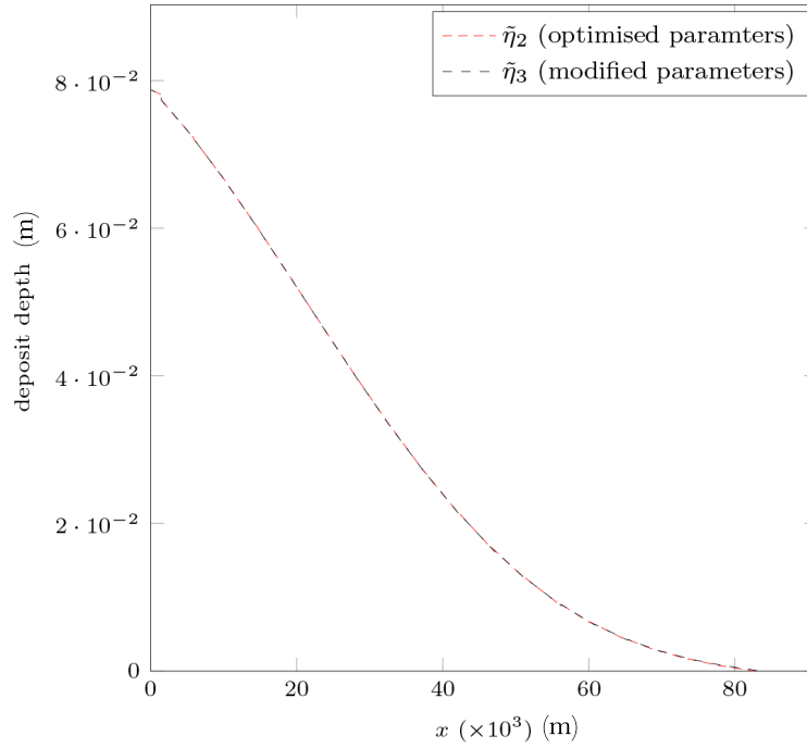
Figure 11. Optimised dimensional deposit output from the model with both mud and sand sediment classes, \tilde{\eta}_2 shown against results from the same model, with the same parameters but a mud settling velocity reduced by two orders of magnitude, \tilde{\eta}_3 .
