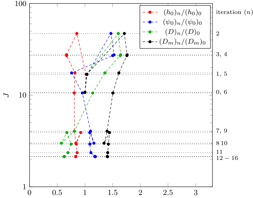
Figure 9. Values of parameters from the model with both mud and sand sediment classes over the optimisation iterations against the value of the objective functional, J , that we are aiming to minimise. Values shown are normalised by their starting values. (*)_n is the value of parameter * at the start of iteration n .
