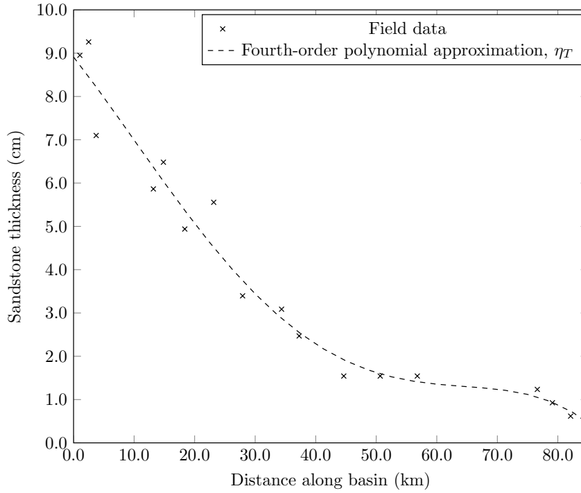
Figure 5. Sandstone depths measured for Bed 1.1 along the Pietralunga and Ridracoli structural elements orientated approximately parallel to the palaeoflow. This has been reconstructed from Figure 5 in Talling et al. (2007a). A fourth-order polynomial approximation of the deposit profile, \eta^T is also shown. This is used as a target for the optimisation algorithm. The base of the bed is shown as a horizontal datum in order to illustrate lateral changes in deposit thickness. Note that a different datum is used in the source figure, which uses the top of Bed 1.2.2 rather than the top of Bed 1. The palaeo-elevation of the base of the bed would have varied spatially, reflecting basin-floor relief.
