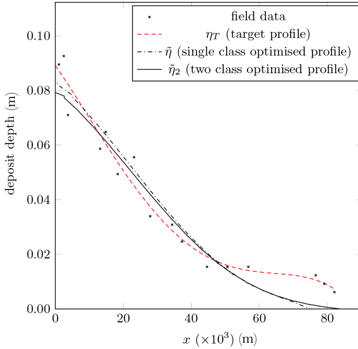
Figure 10. Optimised dimensional deposit output from the model with both mud and sand sediment classes, \tilde{\eta}_2 shown against the optimised results from the single sediment class model, \tilde{\eta} , the field measurement from Bed 1.1 (Talling et al., 2007a) and fourth-order polynomial target deposit profile, \eta^T .
