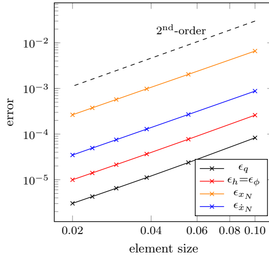
Figure 3. Similarity convergence analysis. All variables are shown to converge on the correct solution at the correct order. \epsilon_{(*)} indicates the L_2 -norm of the error in the solution obtained for variable (*).
