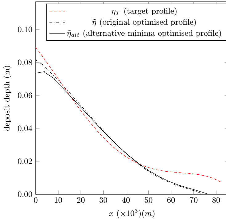
Figure 8. Dimensional deposit output \tilde{\eta} from the optimised deposit output from initial parameter guess (73), and dimensional deposit output \tilde{\eta}_{alt} from an alternative minima achieved by using initial parameter guess (77), shown against the fourth-order polynomial target deposit profile, \eta_T .
