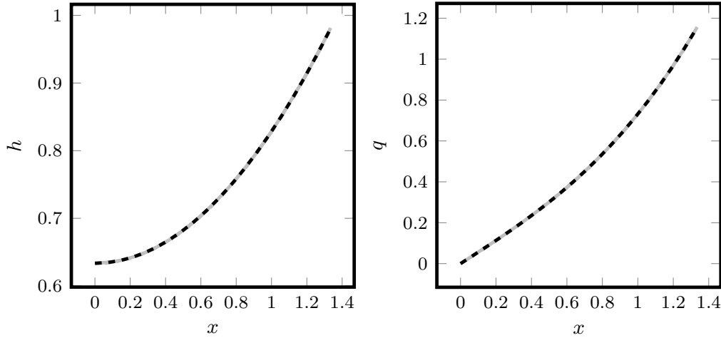
Figure 4. Similarity results for the finest resolution mesh (solid lines), compared against the analytical results (dashed lines) at t = 10.0 .
