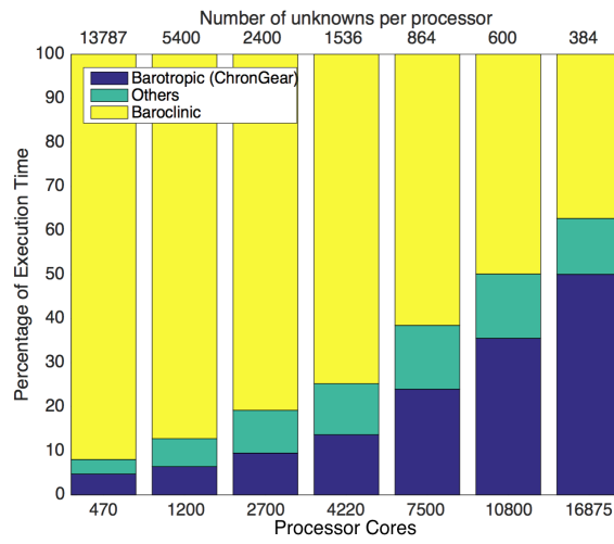
Figure 3. Number of unknowns per processor and percentage of execution time in 0.1^\circ POP using the default diagonal-preconditioned ChronGear solver on Yellowstone.
